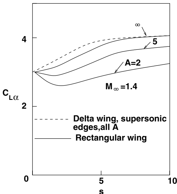
Figure 4.12. Time history of lift curve slope.
