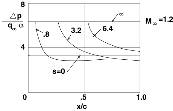
Figure 4.10. Chordwise lifting pressure distribution.
