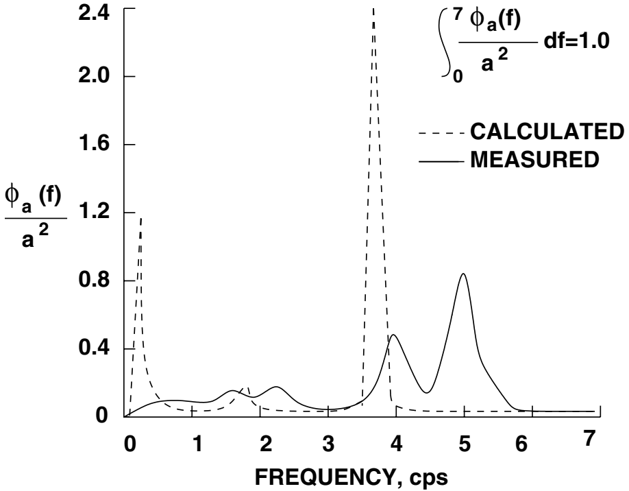
Figure 3.32. Acceleration power spectral density. From Stenton [26].
