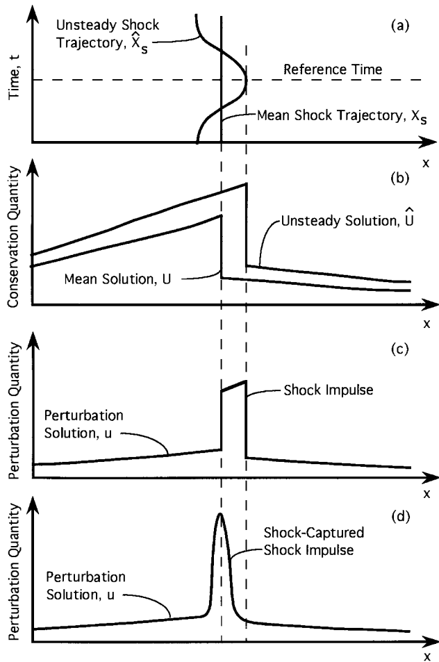
Figure 13.1. Trajectory of shock in a channel or on airfoil surface and corresponding effect on unsteady flow quantities.
