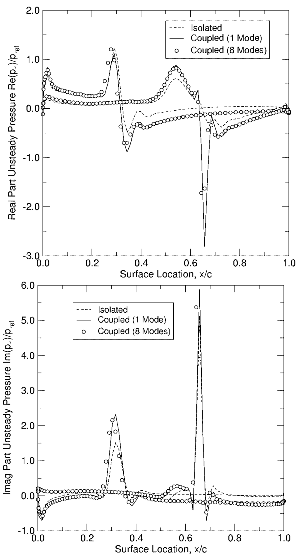
Figure 13.8. Unsteady pressure distribution on the surface of rotor blades vibrating in first bending with \sigma = -30.^\circ
