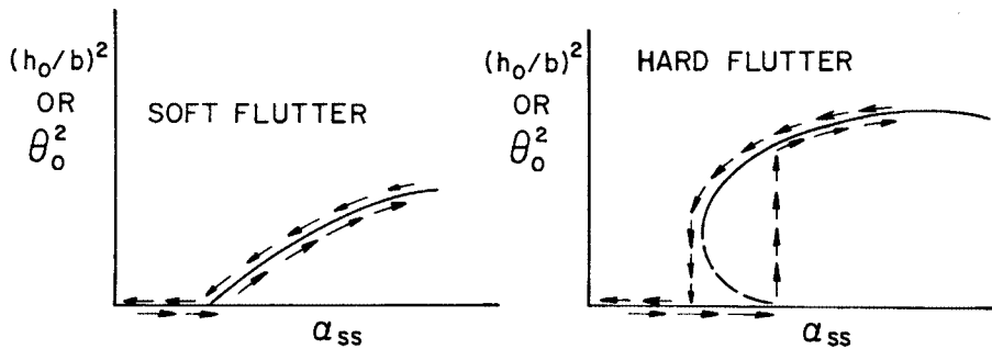
Figure 5.4. Flutter amplitude vs steady state angle of attack.
