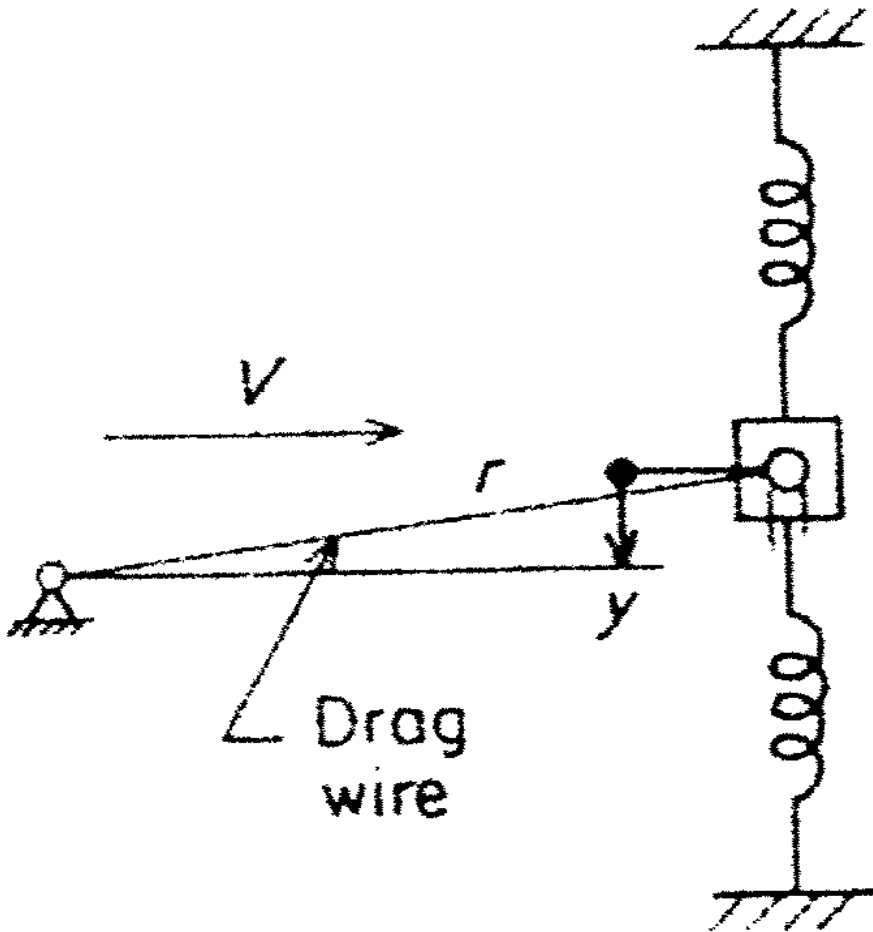
Figure 6.14. Schematic of single galloping oscillator.
