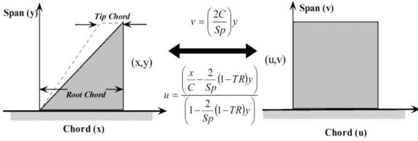
Figure 12.11. Coordinate transformation from dimensionalized rectangular to non-dimensional trapezoidal domain.
