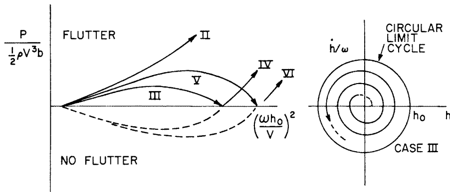
Figure 5.2. Power vs. amplitude.
