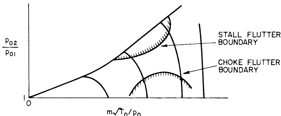
Figure 8.10. Stall flutter boundary.
