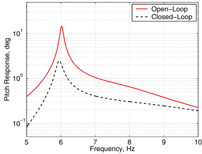
Figure 12.21. Open and Closed loop gain from a force disturbance in plunge to motion in the pitch axes for the typical section model at U = 23 m/s near the open-loop flutterboundary of U_f = 23.4 m/s
