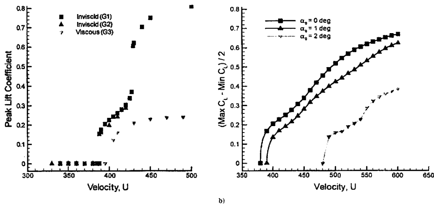
Figure 11.24. LCO Response vs Flow Velocity. An Example of Hysteresis for Goland Wing
