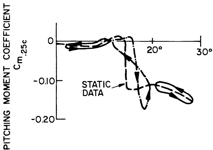
Figure 7.14. Typical oscillating airfoil data [35].
