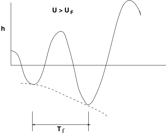
Figure 3.9. Time history of unstable motion or "flutter".
