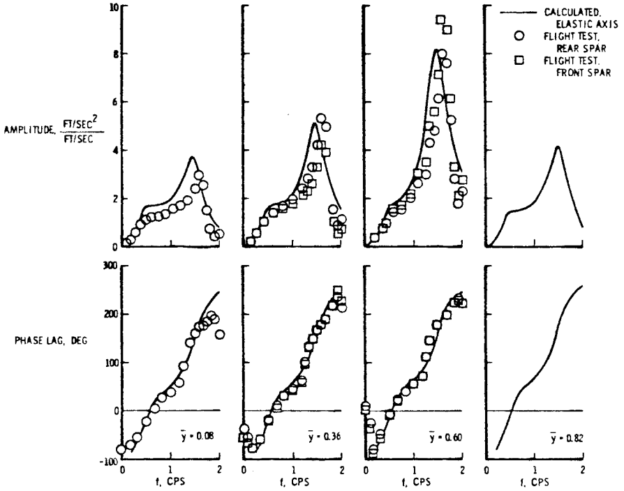
Figure 3.33. \bar{y} = nondimensional distance along span. From Houbolt [6].
