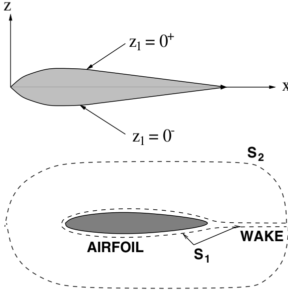
Figure 4.5. Airfoil and flow field geometry.
