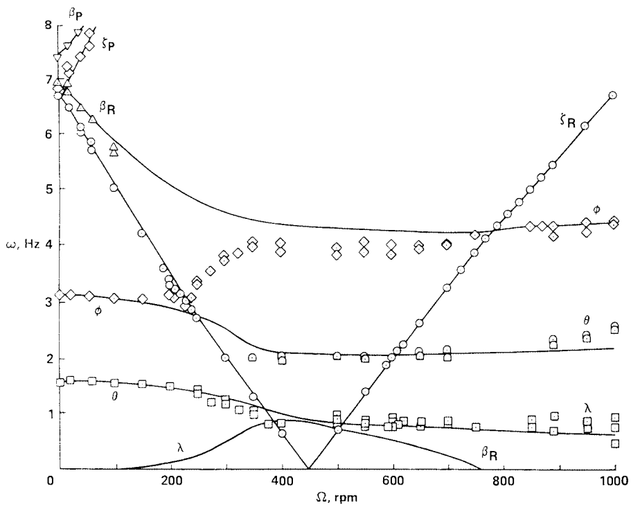
Figure 7.29. Influence of Unsteady aerodynamics on hingeless rotor ground resonance. Comparison of measured modal frequencies, and calculations including dynamic inflow.
