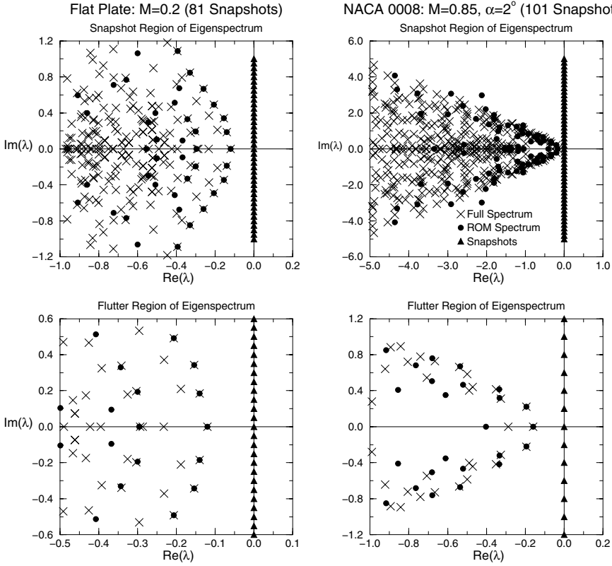
Figure 9.6. A comparison of the full and ROM aerodynamic eigenspectrums. \text{Re}(\lambda) , real eigenvalues; \text{Im}(\lambda) , imaginary eigenvalues; M, Mach number; \alpha , angle of attack. (Republished from Thomas et al (1999) with permission.)
