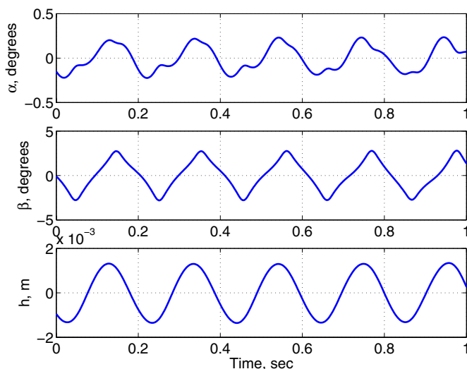
Figure 12.10. Limit cycle behavior of nonlinear system at 30% of linear flutter speed
