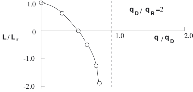
Figure 2.5. Lift vs dynamic pressure.
