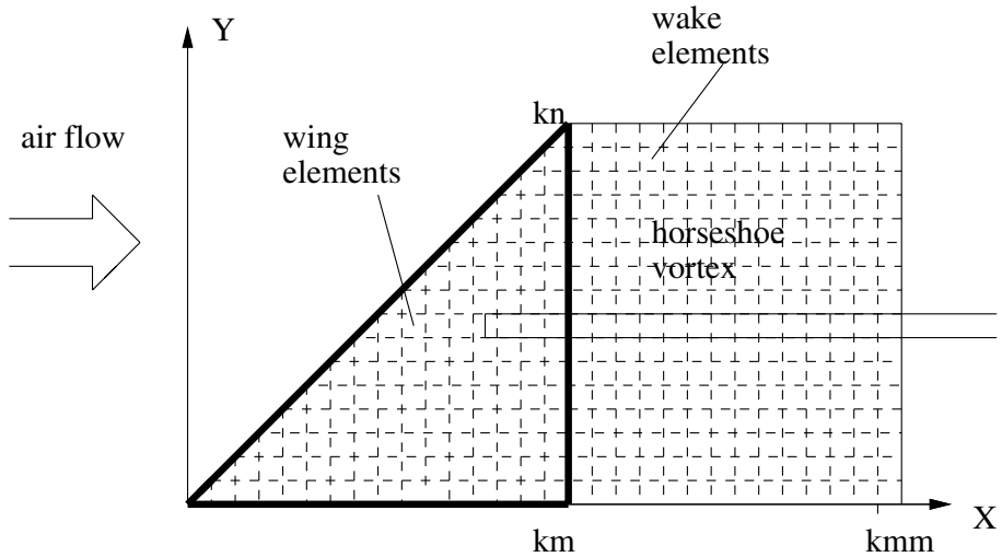
Figure 9.21. Aeroelastic model of delta wing using vortex-lattice aerodynamic model. (Republished with permission from Tang et al (1999).)
