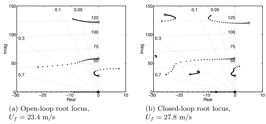
Figure 12.22. Root Loci as flowspeed is varied from 0 m/s (Circle) to 30 m/s (X). The closed-loop system is unstable below 11.2 m/s and above 27.8 m/s
