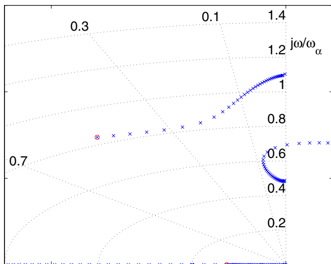
Figure 12.8. Root locus showing variation of system eigenvalues with reduced order aerodynamic model, parameters chosen as in [19]
