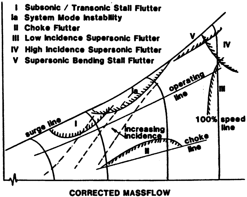
Figure 8.13. Axial compressor or fan characteristic map showing principle types of flutter and region of occurrence.
