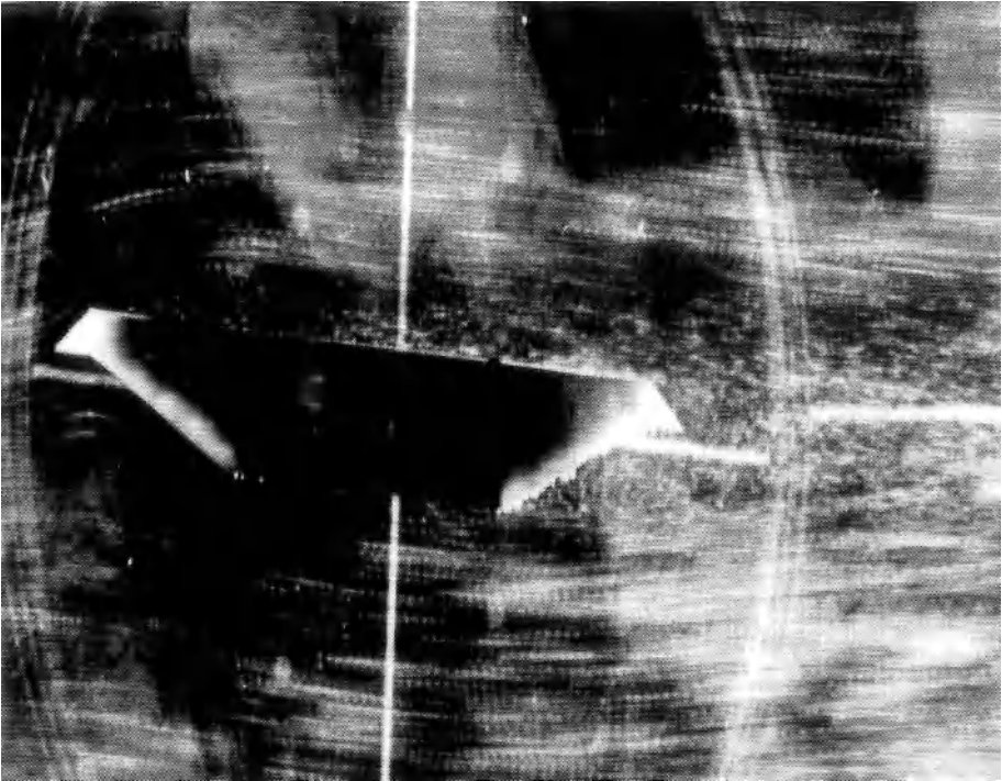
Figure 6.30b. Visualization of water flow over a partially streamlined bridge model deck section (courtesy of the National Aeronautical Establishment, National Research Council of Canada).
