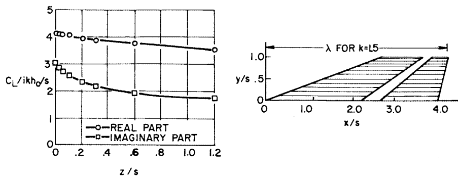
Figure 4.13. Lift coefficient of plunging wing-tail combination for various vertical separation distances; simple harmonic motion.
