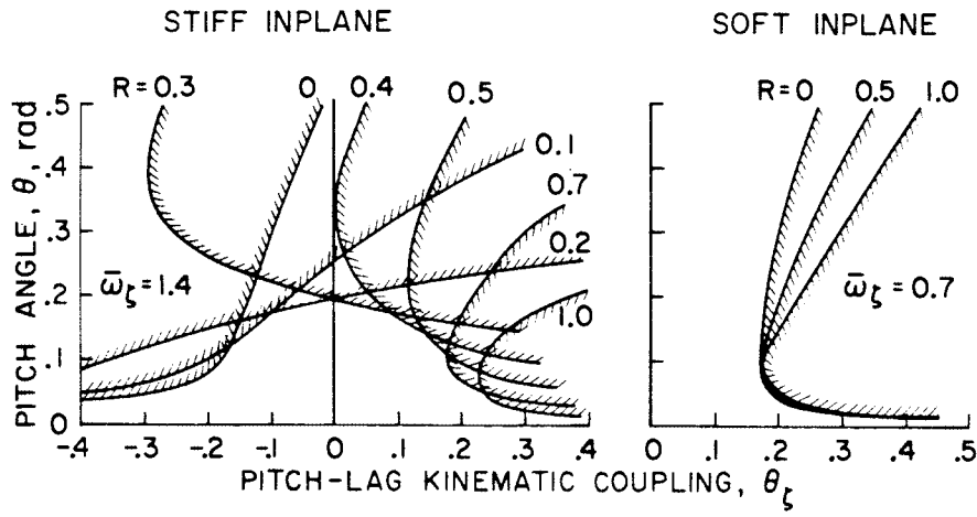
Figure 7.12. Flap-lag stability boundaries as a function of pitch-lag coupling and elastic coupling [17].
