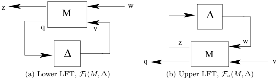
Figure 12.2. Linear Fractional Transformation of \Delta on M
