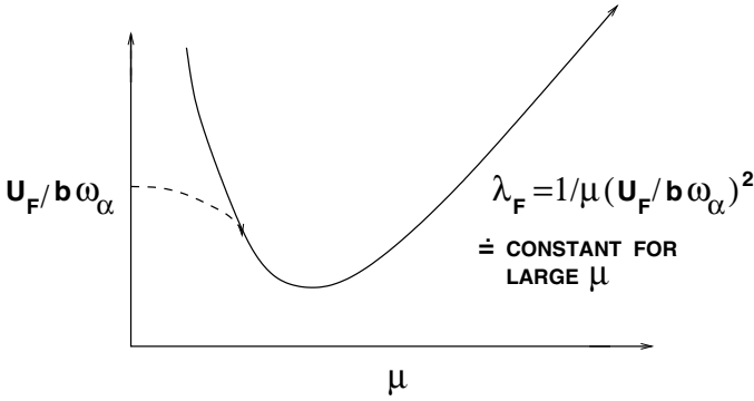
Figure 3.27. Flutter air speed vs mass ratio.
