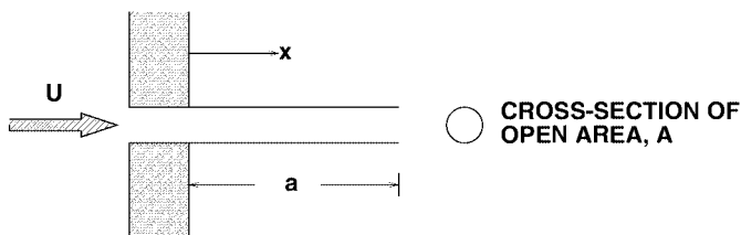
Figure 3.39. Geometry of pipe.
