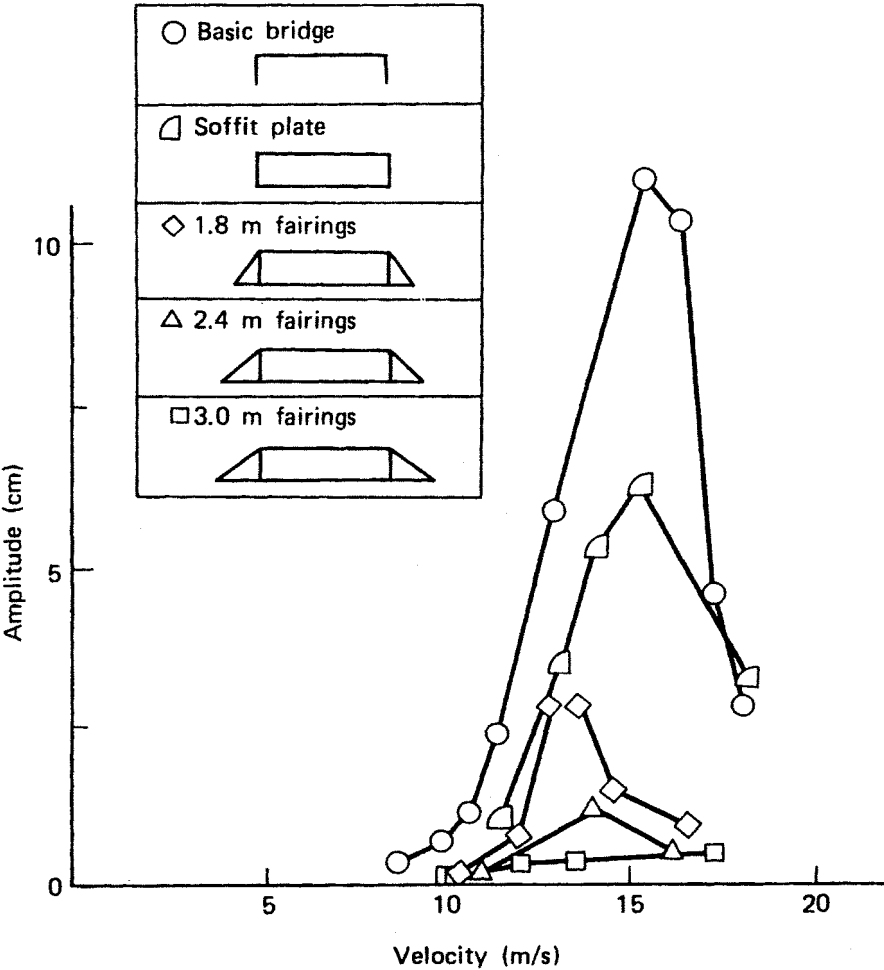
Figure 6.29. Vertical amplitudes of vortex-induced deflections for various bridge deck sections of the proposed Long Creek’s bridge [65] (courtesy of the National Aeronautical Establishment, National Research Council of Canada).
