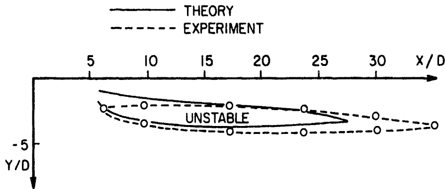
Figure 6.19. Measured and predicted stability boundaries for wake galloping [43].
