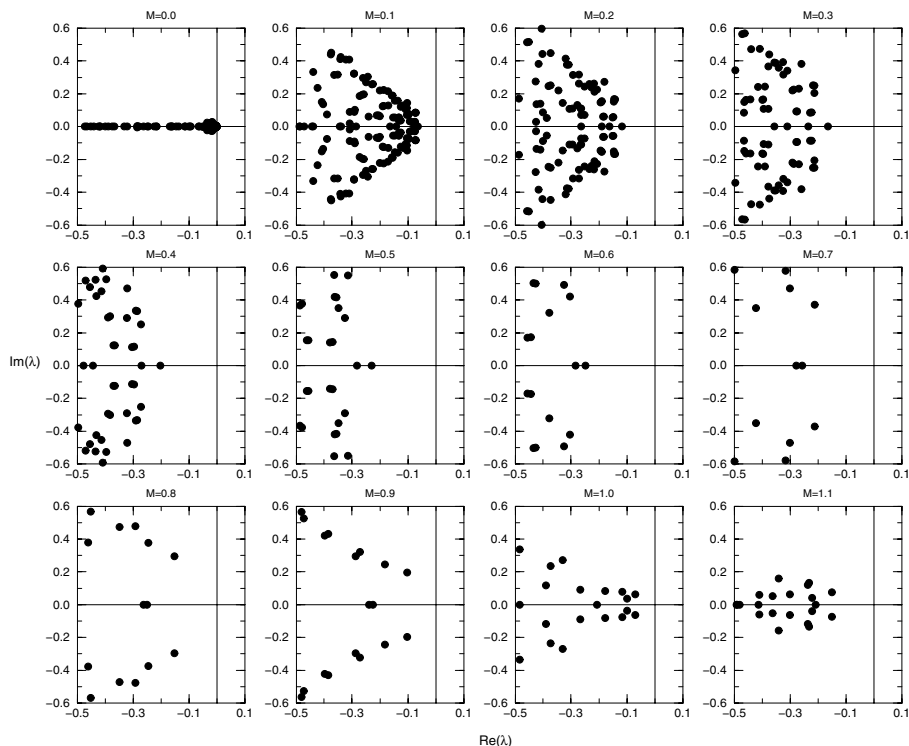
Figure 9.5. Full aerodynamic eigenspectrums. Re, real; Im, imaginary, M, Mach number. Flat-plate airfoil ( 16 \times 8 mesh). (Republished from Thomas et al (1999) with permission.)
