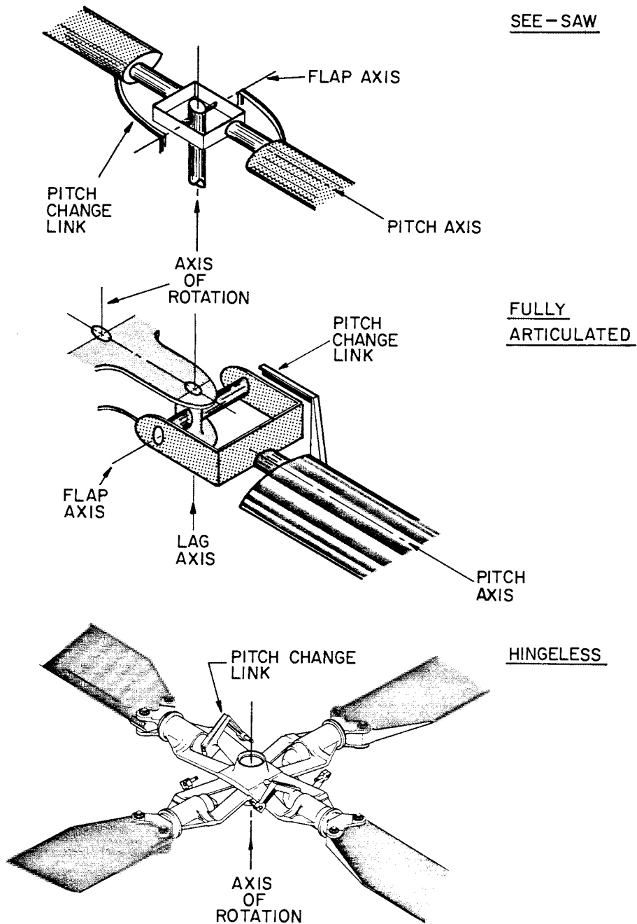
Figure 7.1. Various rotor hub configurations.
