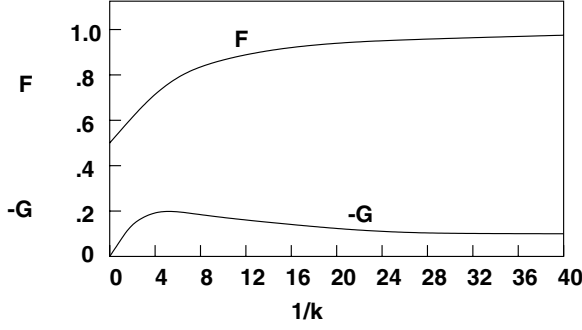
Figure 4.6. The functions F and G against \frac{1}{k} . After Theodorsen [19].
