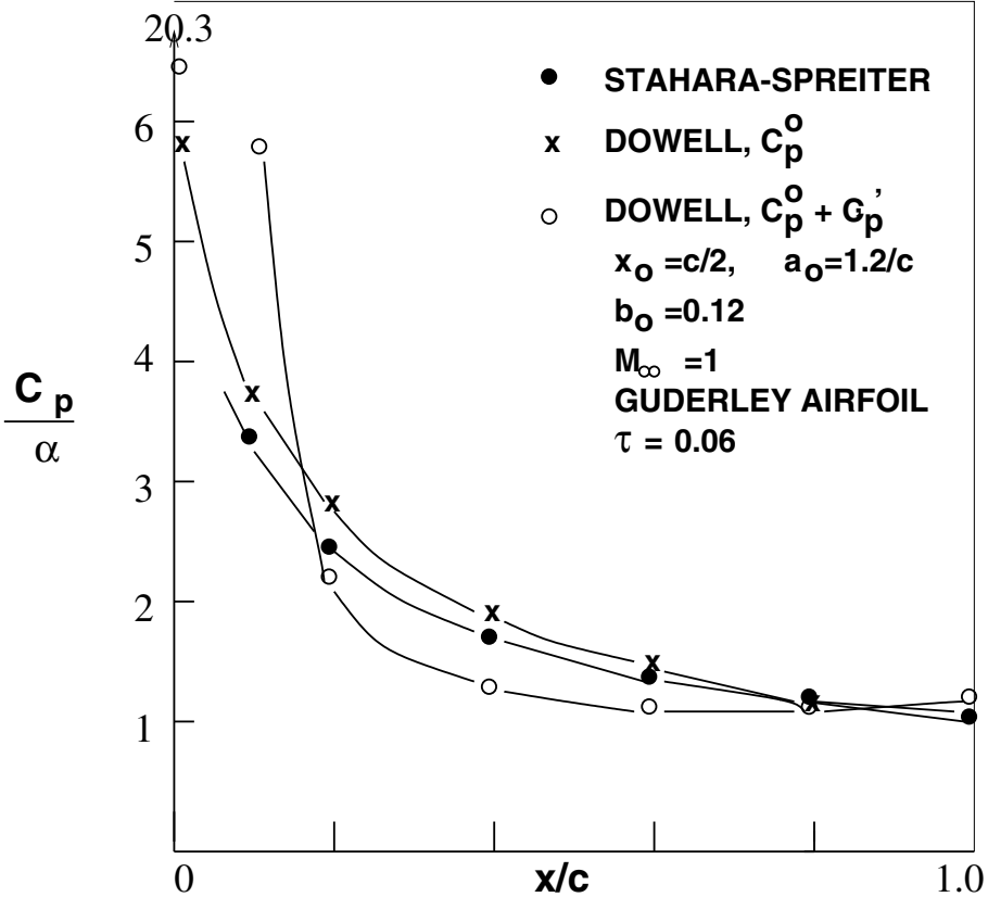
Figure 4.18. Pressure distribution for Guderley airfoil at constant angle of attack.
