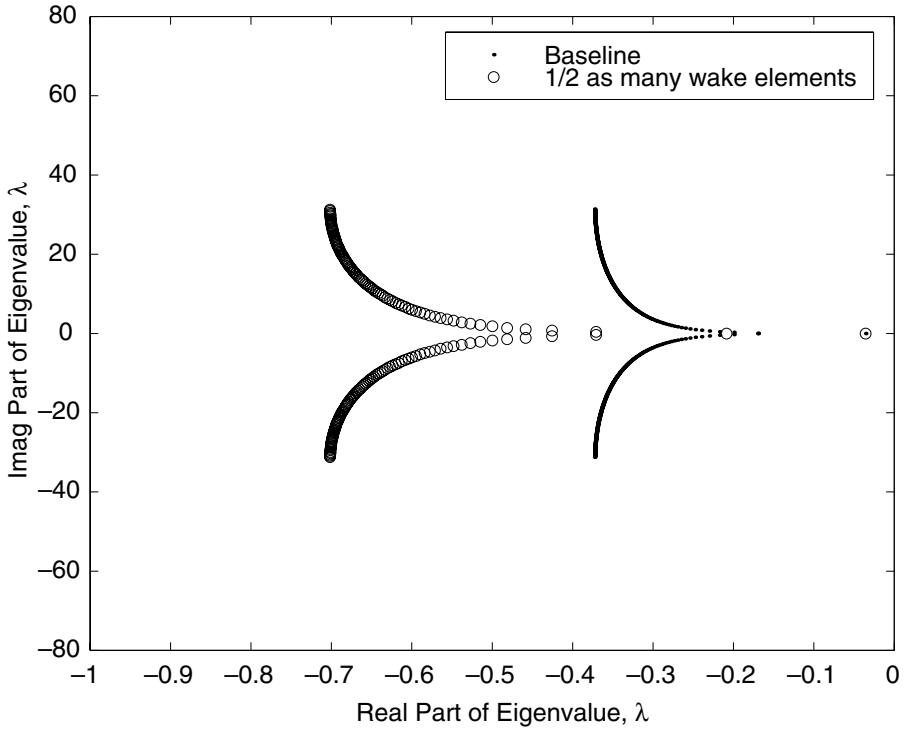
Figure 9.4. Influence of varying the number of aerodynamic elements in the wake of the vortex-lattice model, while maintaining the element size. Shown are continuous-time real and imaginary (Imag) eigenvalues, \lambda . (Republished from Heeg & Dowell (1999) with permission.)
