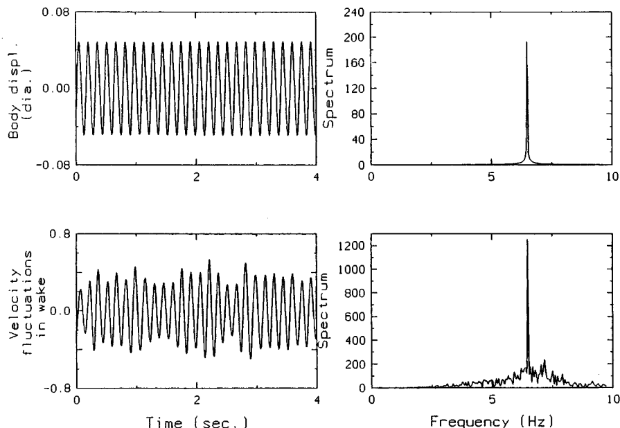
Figure 6.5b. Response for U/f_n D = 5.003 ; \zeta = 0.15\% .
