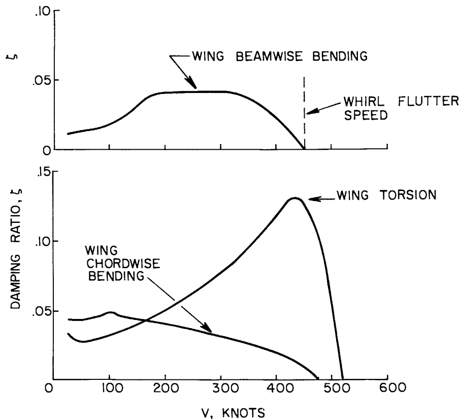
Figure 7.27. Damping of wing bending modes as a function of airspeed. Tilt prop/rotor aircraft with gimballed rotor [6].
