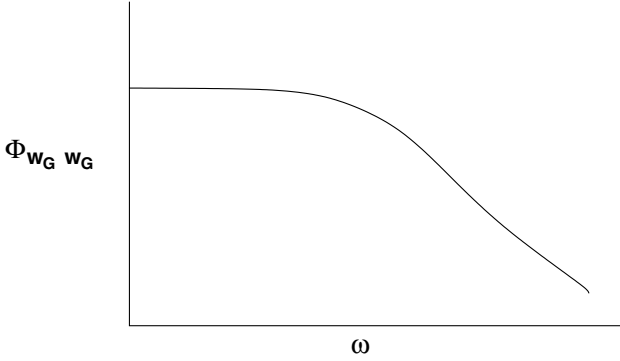
Figure 3.5. Gust (auto) power spectral density.
