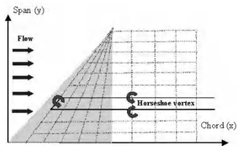
Figure 12.14. Vortex lattice construction grid for wing and wake.
