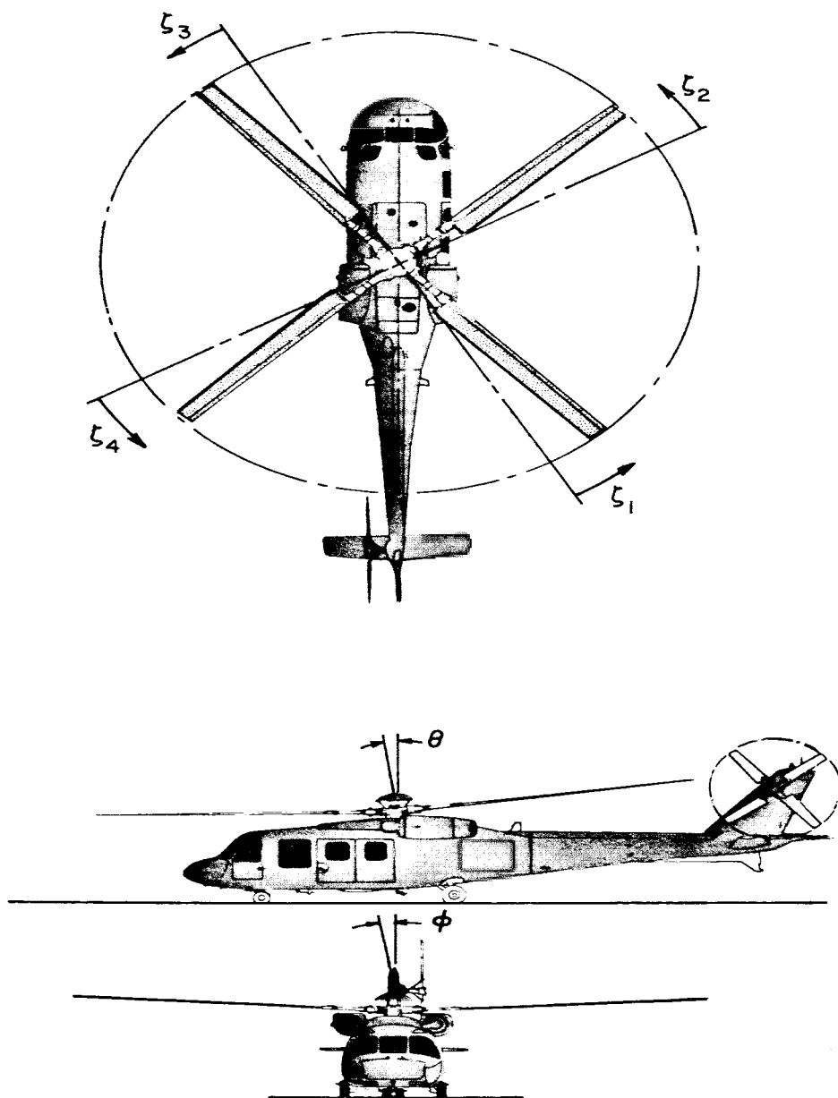
Figure 7.16. Mechanical degrees of freedom for ground resonance analysis.
