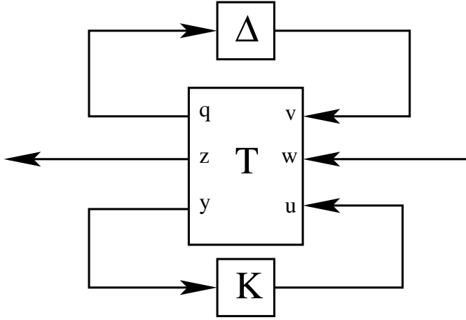
Figure 12.3. General LFT framework for linear robust control problems
