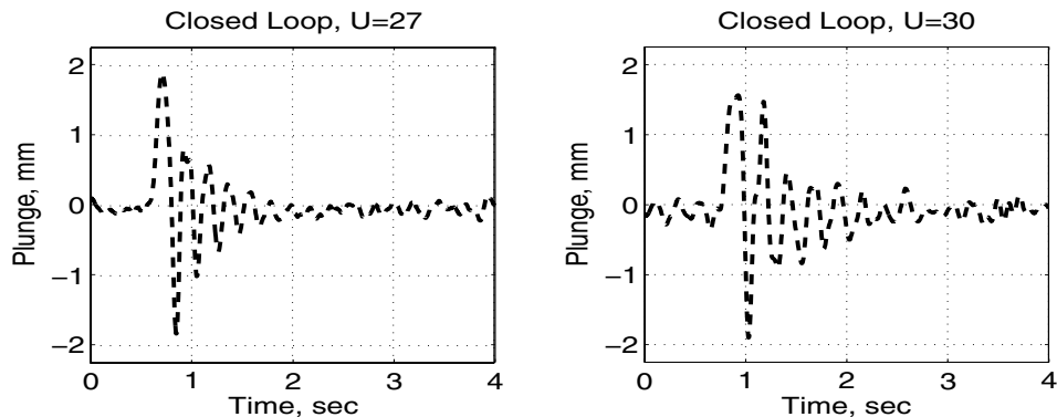
Figure 12.28. Closed loop disturbance response in plunge for flow conditions above the open-loop flutter boundary
