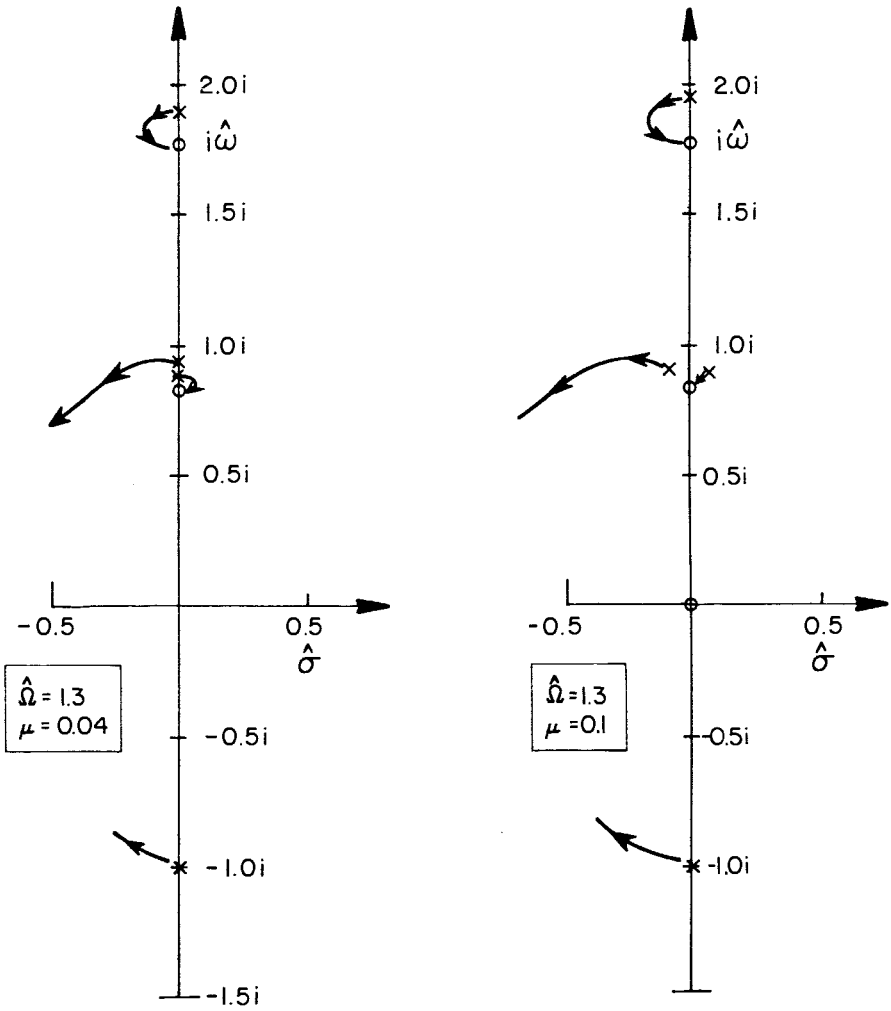
Figure 7.23. Root locus for increasing pylon (fixed axis) damping on ground resonance stability.
