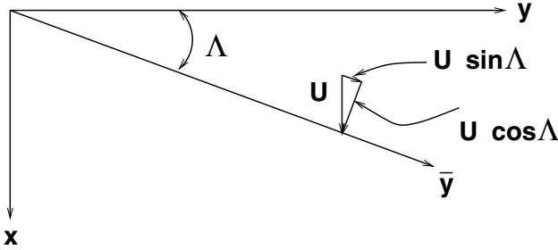
Figure 2.18. Velocity diagram in the x, y(\bar{x}, \bar{y}) plane.
