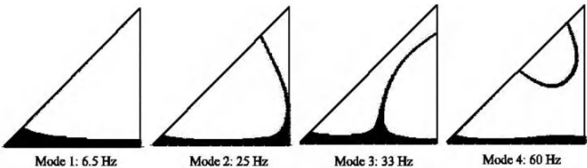
Figure 12.12. Invacuo mode shape node-line predictions for first four structural modes.
