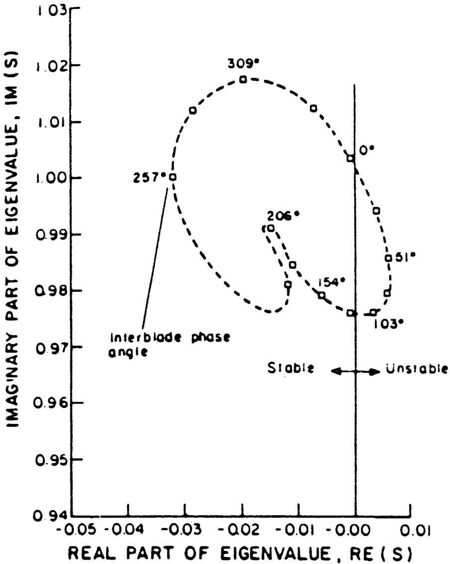
Figure 8.12a. Aeroelastic eigenvalues of a 14-bladed tuned rotor.
