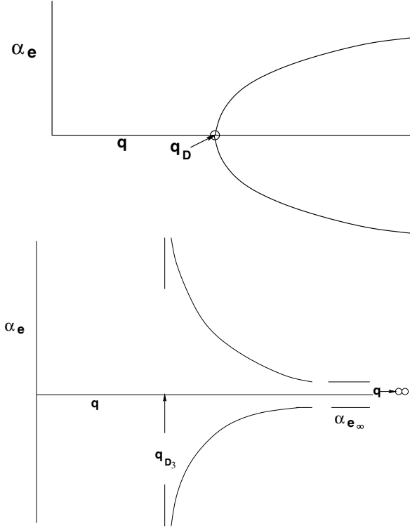
Figure 2.6. (Nonlinear) equilibria for elastic twist: e > 0 . (top) e < 0 . (bottom)
