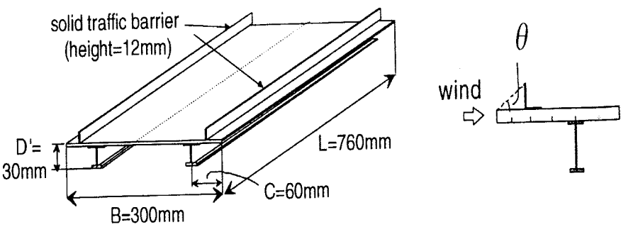
Figure 6.33. A “ \pi -section” deck. From Y. Kubo, K. Sadashima, E. Yamaguchi, K. Kato, Y. Okamoto, T. Koga, “Improvement of aeroelastic instability of shallow \pi section,” J. Wind Eng. Ind. Aerod. 89 (2002) 1445-1457.
