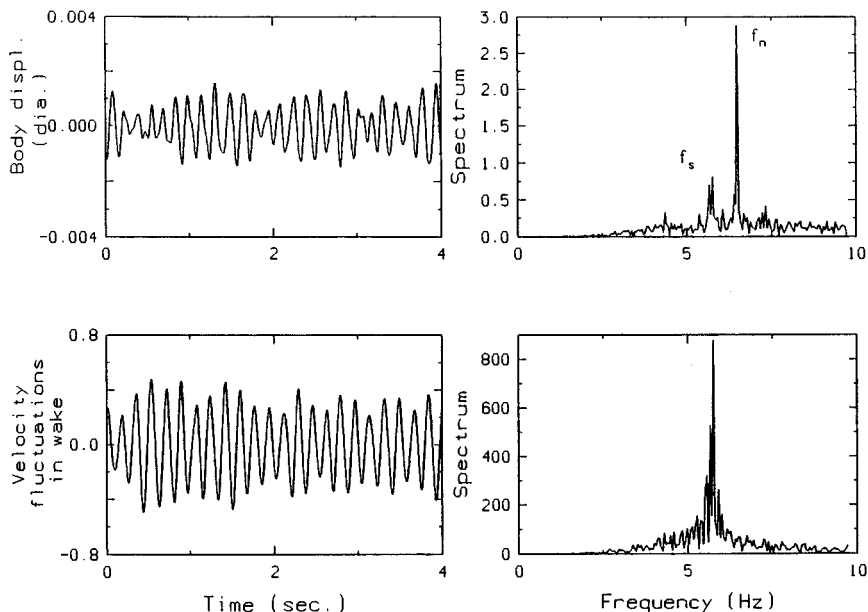
Figure 6.5a. Response for U/f_n D = 4.294 ; \zeta = 0.15\% .
