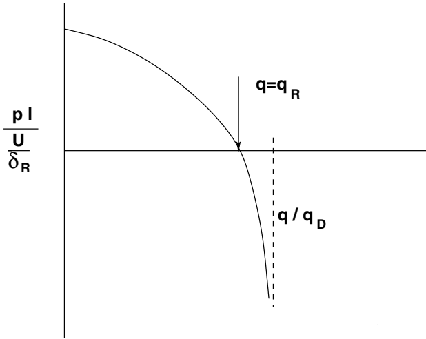
Figure 2.14. Roll rate vs dynamic pressure.
