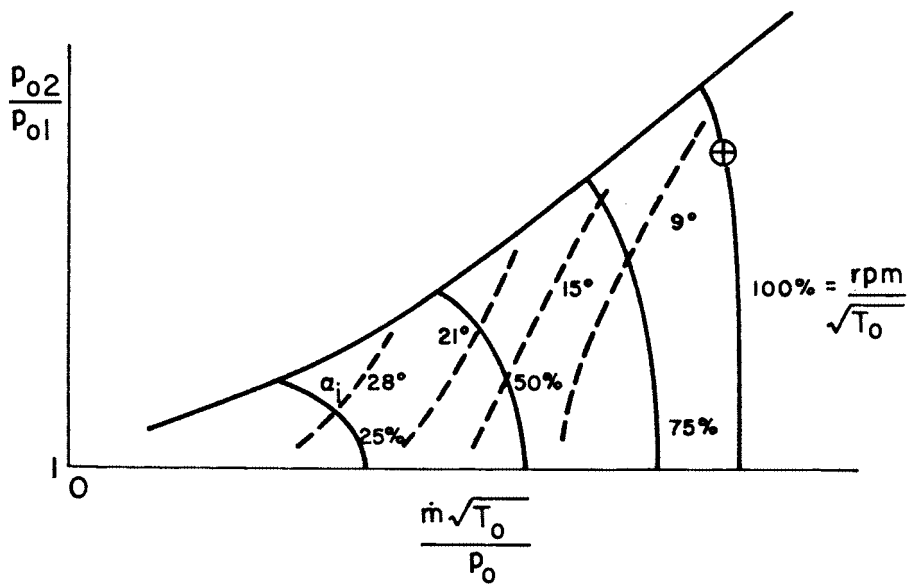
Figure 8.4. Map showing incidence as a parameter.
