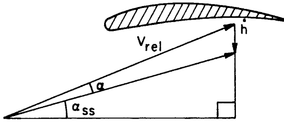
Figure 5.1. Velocity triangle.
