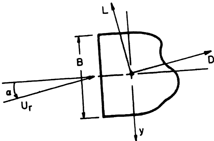
Figure 6.8. Lift L and drag force D on a fixed bluff object.
