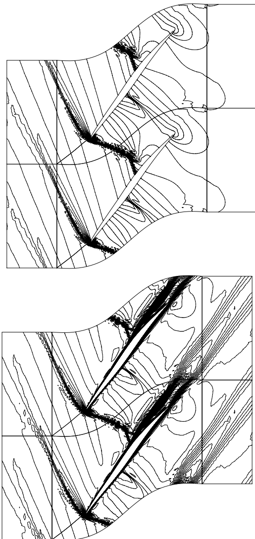
Figure 13.10. Computed steady pressure (top) and Mach number (bottom) contours for transonic viscous flow through front stage compressor rotor.
