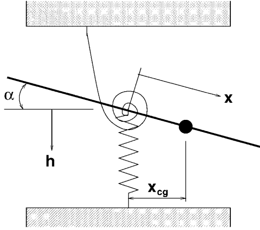
Figure 3.1. Geometry of typical section airfoil.
