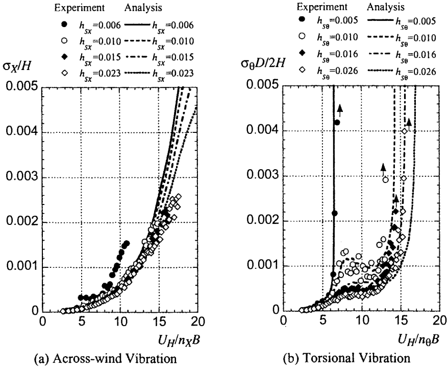
Figure 6.37. Displacements of wind response obtained from response analysis accounting for measured aerodynamic damping and from wind tunnel tests on elastic model; shear flow corresponding to suburban terrain. From J. Katagiri, T. Okhuma, and H. Marukawa, "Motion-induced wind forces acting on rectangular high-rise buildings with side ratio of 2," J. Wind Eng. Ind. Aerod. 89 (2001) 1421-1432.
