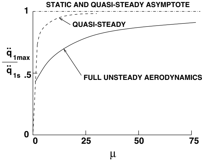
Figure 3.38. Maximum acceleration for wing in translation encountering a sharp edge (step function) gust as given by various aerodynamic models vs mass ratio.
