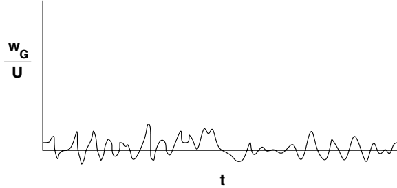
Figure 3.10. Time history of stable motion.
