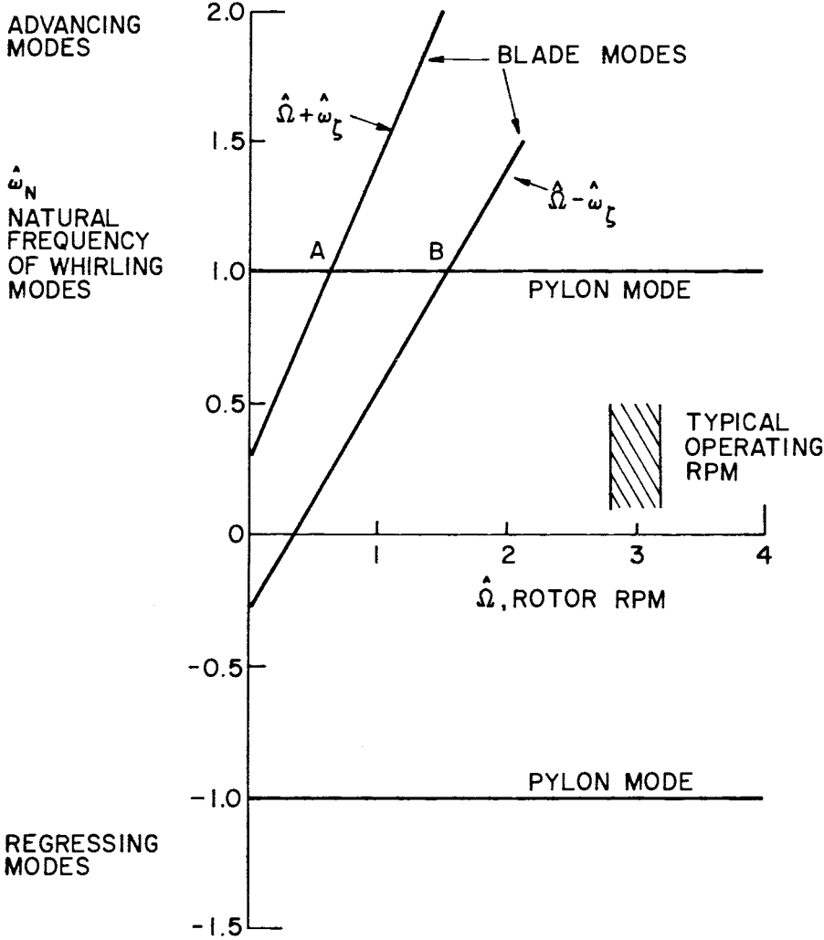
Figure 7.19. Uncoupled whirling modes ( \mu = 0 ). Fixed coordinate system.
