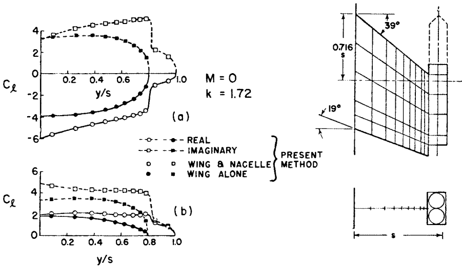
Figure 4.15. Distribution of span load for wing with and without engine nacelle. (a) plunging (b) pitching; simple harmonic motion.
