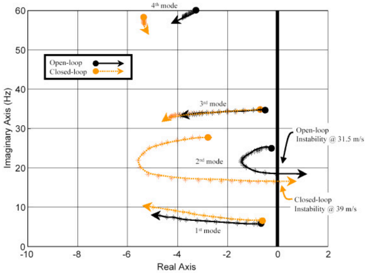
Figure 12.23. Closed-loop aeroelastic root migrations.
