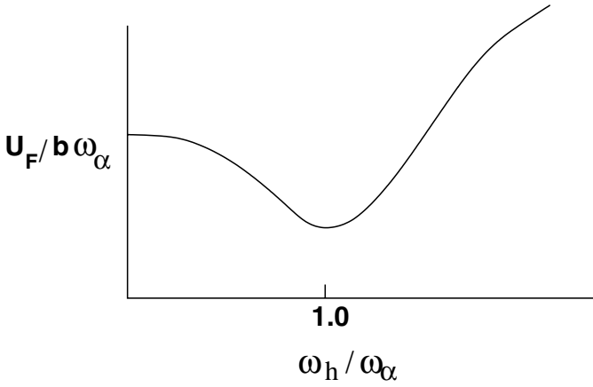
Figure 3.24. Flutter airspeed vs frequency ratio.
