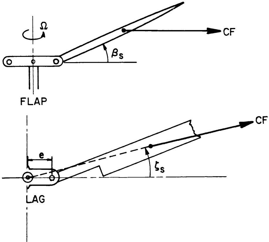
Figure 7.3. Direction of centrifugal force for flap and lag motion.
