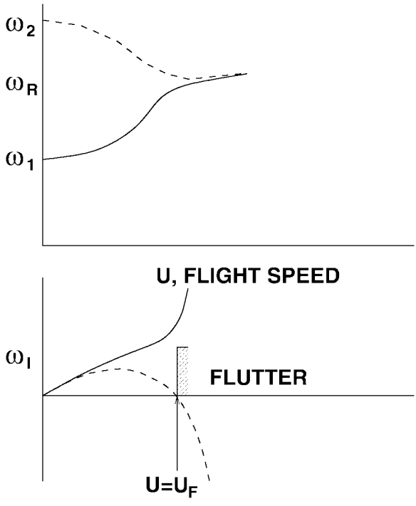
Figure 3.13. Real and imaginary components of frequency vs air speed.
