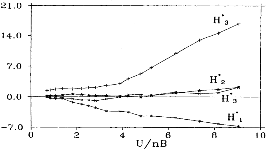
Figure 6.26. Aerodynamic coefficients H_i^* ( i = 1, 2, 3, 4 ), Golden Gate Bridge (courtesy of Dr. J. D. Raggett, West Wind Laboratory, Carmel, CA).
