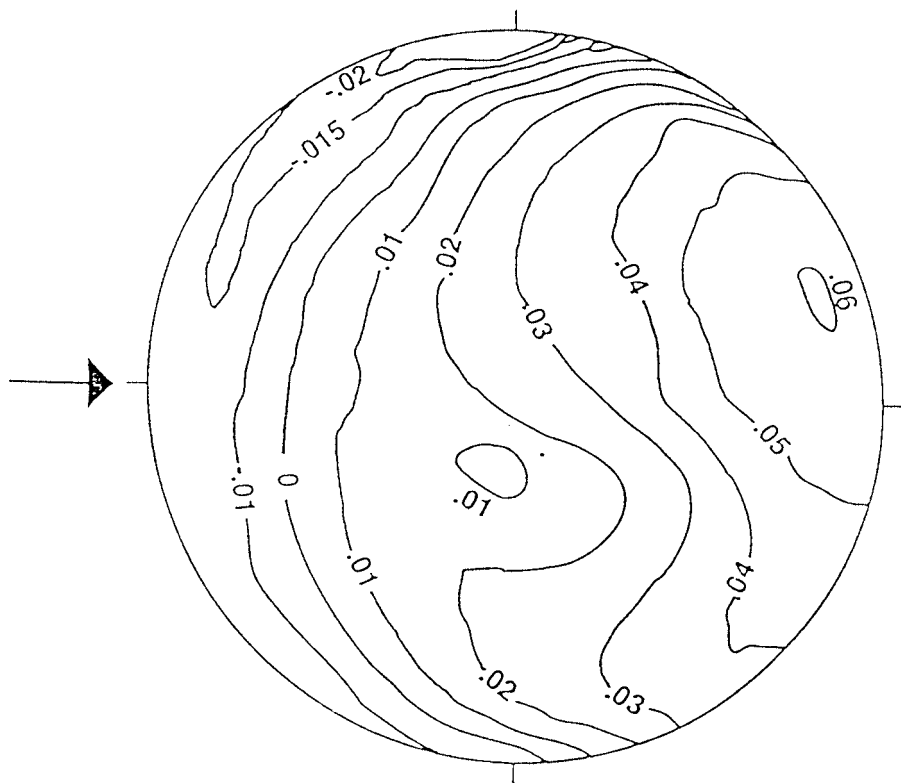
Figure 7.30. Experimental induced inflow distribution. Tapered blade, \mu = 0.15 .
