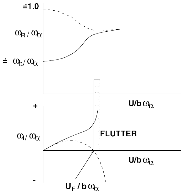
Figure 3.17. Real and imaginary components of frequency vs air speed.
