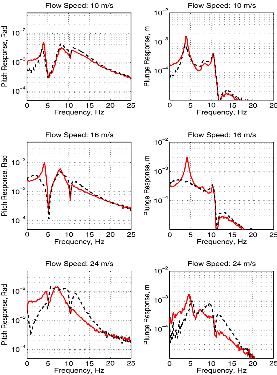
Figure 12.31. Comparison of open (solid) and closed (dashed) loop transfer functions from spectral data with flap excitation.
