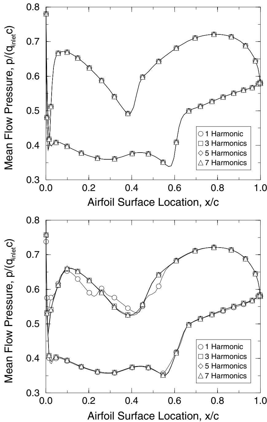
Figure 13.11. Zeroth harmonic (mean flow) of unsteady pressure distribution for front stage compressor rotor airfoils vibrating in pitch with \overline{\omega} = 1.0 and \sigma = 30^\circ , and \overline{\alpha} = 1.0^\circ .
