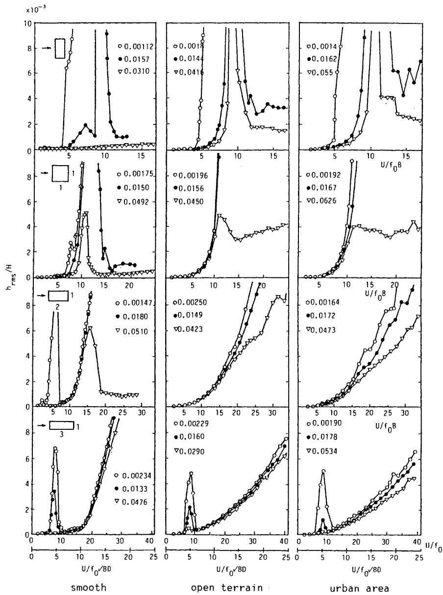
Figure 6.36. Wind tunnel measurements of across-wind response of rectangular buildings (circles and triangles indicate damping ratios). From H. Kawai, "Vortex Induced Vibration of Tall Buildings," J. Wind Eng. Ind. Aerod. 41-44 (1993) 117-128.
