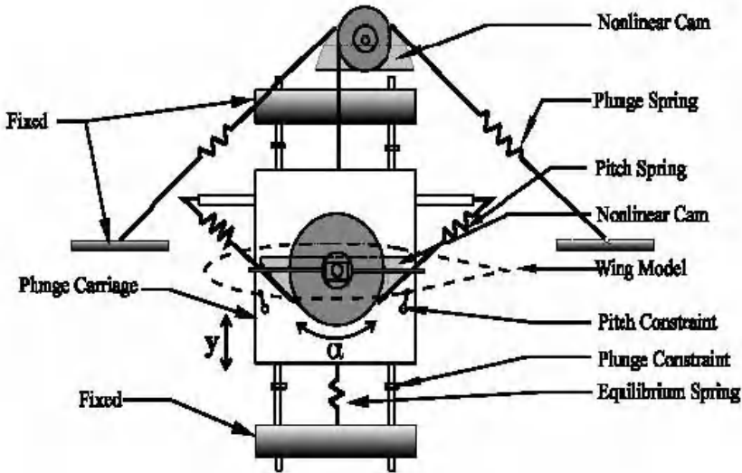
Figure 11.11. The Nonlinear Aeroelastic Test Apparatus (NATA) in Texas A&M's 2'x3' Wind Tunnel
