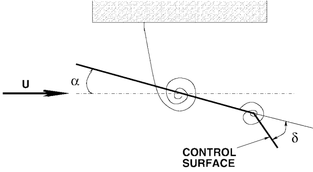
Figure 2.4. Typical section with control surface.
