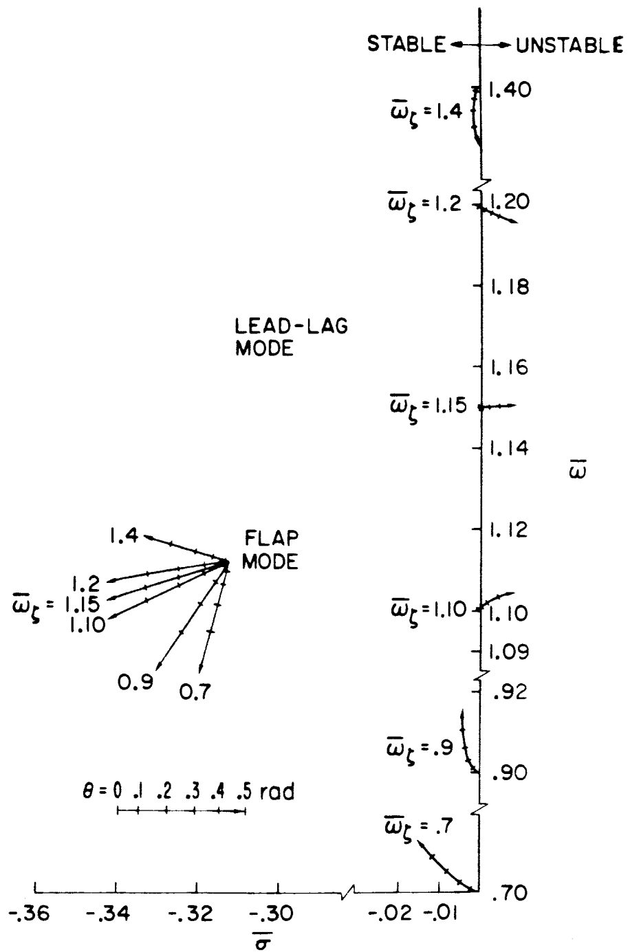
Figure 7.9. Locus of roots for increasing blade pitch. R = 0 , no elastic coupling.
