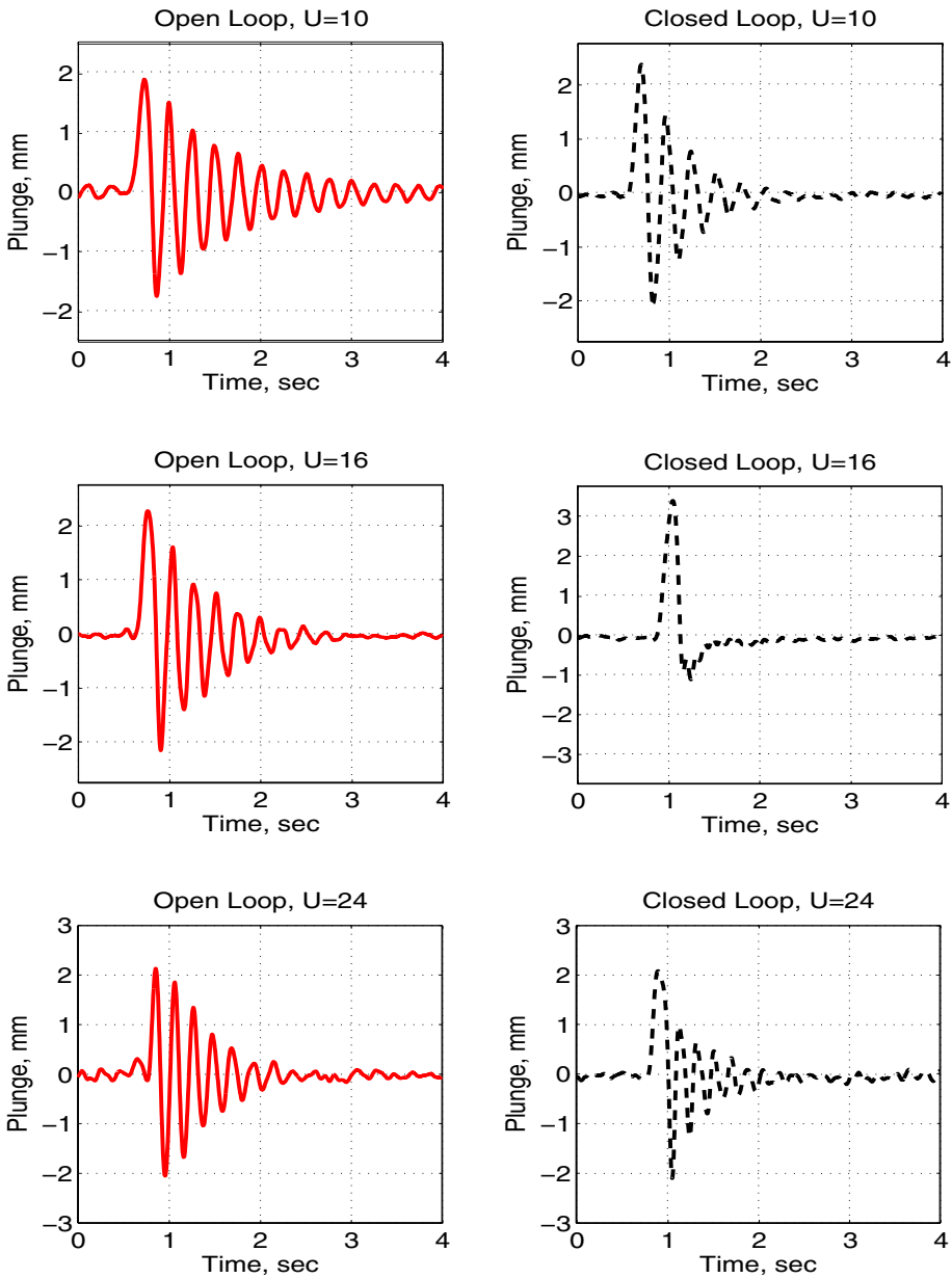
Figure 12.30. Open and Closed loop disturbance response in plunge.
