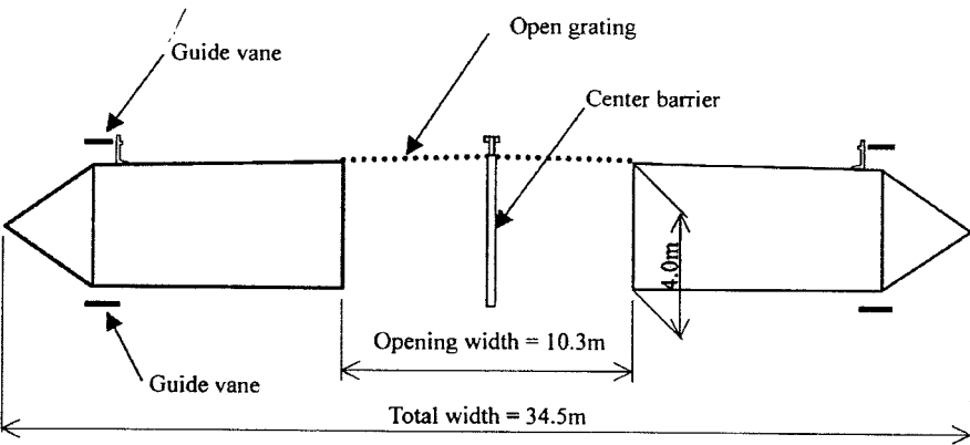
Figure 6.33. A “ \pi -section” deck. From Y. Kubo, K. Sadashima, E. Yamaguchi, K. Kato, Y. Okamoto, T. Koga, “Improvement of aeroelastic instability of shallow \pi section,” J. Wind Eng. Ind. Aerod. 89 (2002) 1445-1457.
