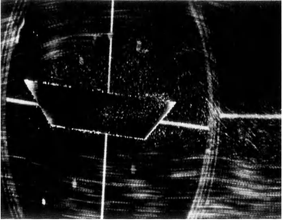
Figure 6.30a. Visualization of water flow over a bridge model deck section (courtesy of the National Aeronautical Establishment, National Research Council of Canada).
