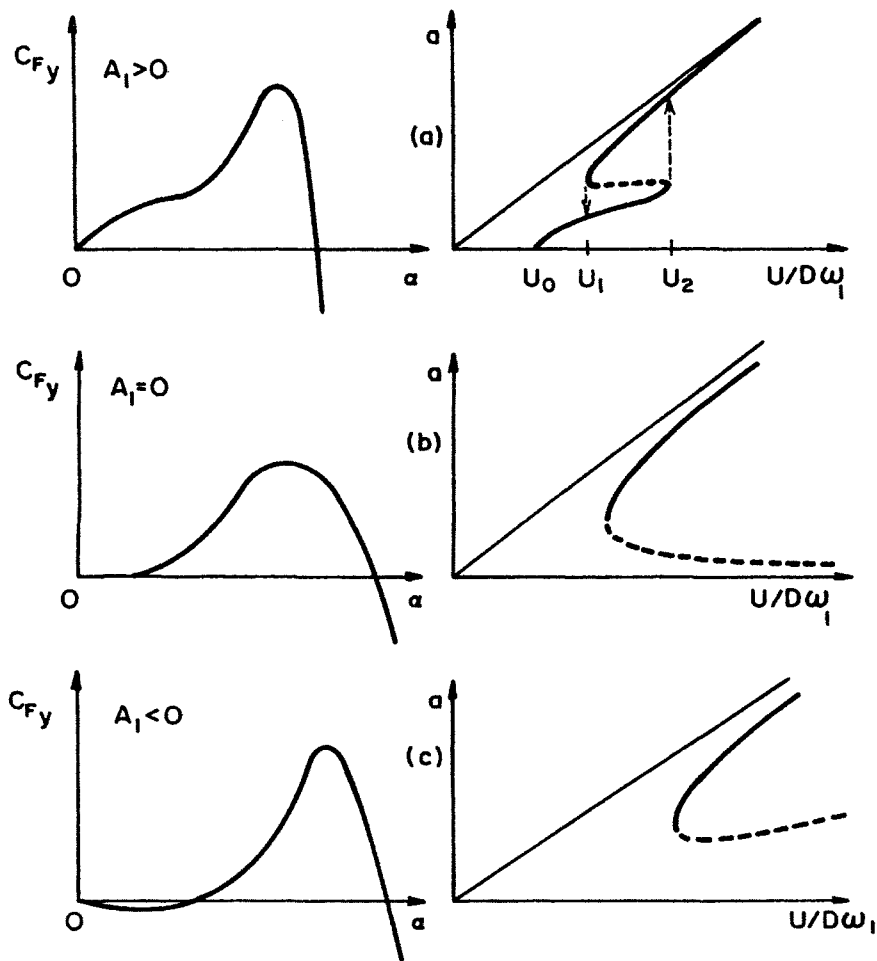
Figure 6.11. Basic types of lateral force coefficients C_{fy} and the corresponding galloping response amplitudes. From M. Novak, "Galloping Oscillations of Prismatic Structures," J. Eng. Mech. Div. , ASCE 98 (1972) 27-46.
