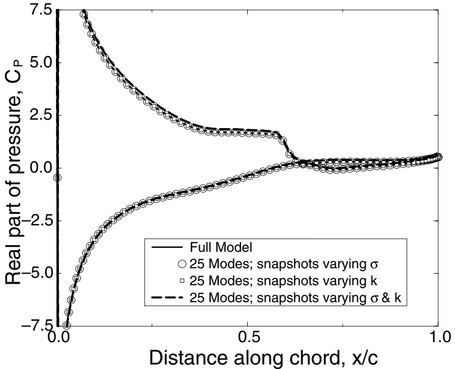
Figure 9.18. Real part of the coefficient of pressure C_p obtained by using 25 POD modes when the interblade phase angle \sigma is 90^\circ , the reduced frequency k is 0.85, and the upwind far-field Mach number M is 0.5. (Republished with permission from Epureanu et al (2001).)
