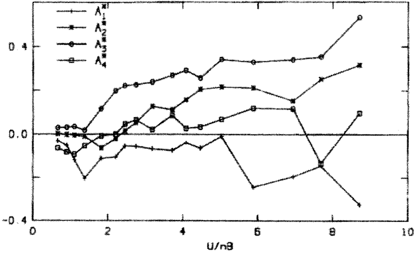
Figure 6.28. A_i^* flutter derivatives of Golden Gate bridge at 5^\circ ( i = 1, 2, 3, 4 ). From A. Jain, N.P. Jones, R.H. Scanlan "Effect of modal damping on bridge aeroelasticity", J. Wind Eng. Ind. Aerod. 77-78 (1998) 421-430.
