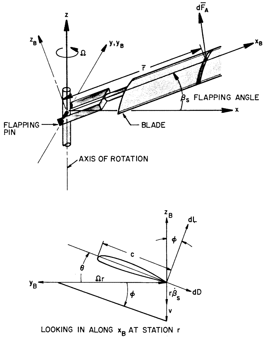
Figure 7.2. Coordinate systems and aerodynamics for blade flapping analysis.
