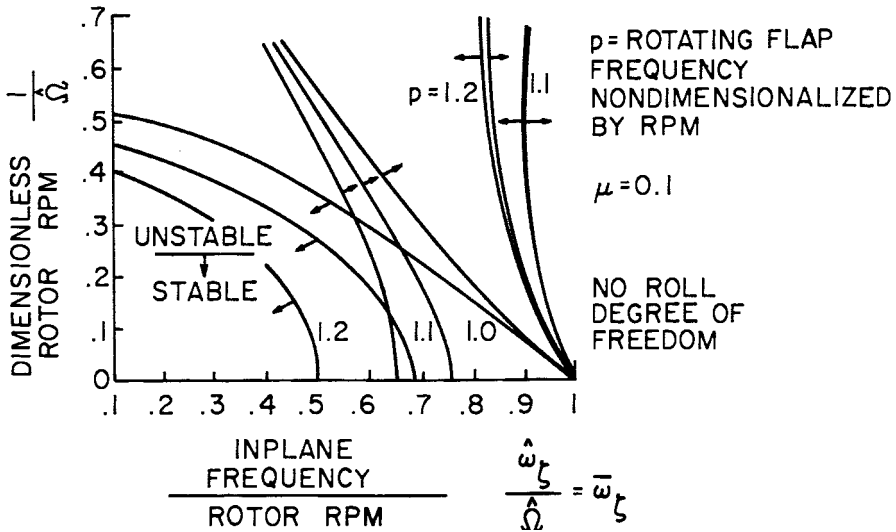
Figure 7.25. Influence of flap frequency on ground resonance stability boundaries [10].
