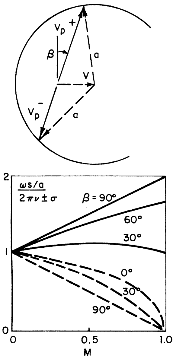
Figure 8.8. Resonant values of governing parameters.
