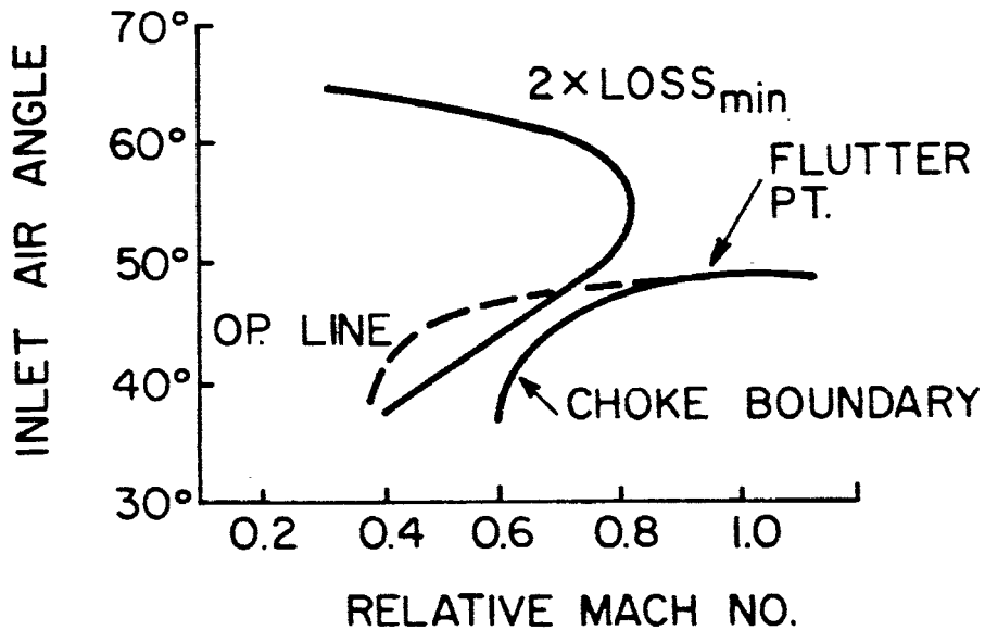
Figure 8.11. Choking flutter correlation.
