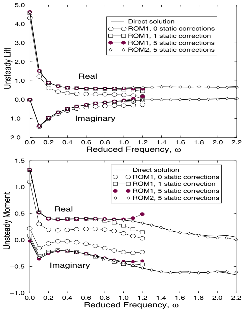
Figure 9.15. Unsteady lift ( top ) and moment ( bottom ) on NACA 0012 airfoil pitching about its midchord ROM, reduced-order model. Mean flow conditions: \theta = 2^\circ , M_\infty=0.75 . Locally refined grid. (Republished from Florea et al (1999) with permission.)
