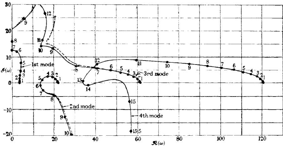
Figure 3.40a. The dimensionless complex frequency of the four lowest modes off the system as a function of the dimensionless flow velocity for \beta = 0.200 . —, Exact analysis — four-mode approximation (Galerkin). Numbers on graph are values of u .
