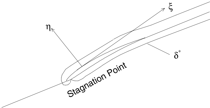
Figure 9.17. Solution domain used to calculate the inviscid flow. Special local analytic solution is used at the stagnation point. The system of coordinates along the airfoil surface is indicated by \xi and \eta . A typical displacement thickness is sketched along the airfoil and wake. (Republished with permission from Epureanu et al (2001).)
