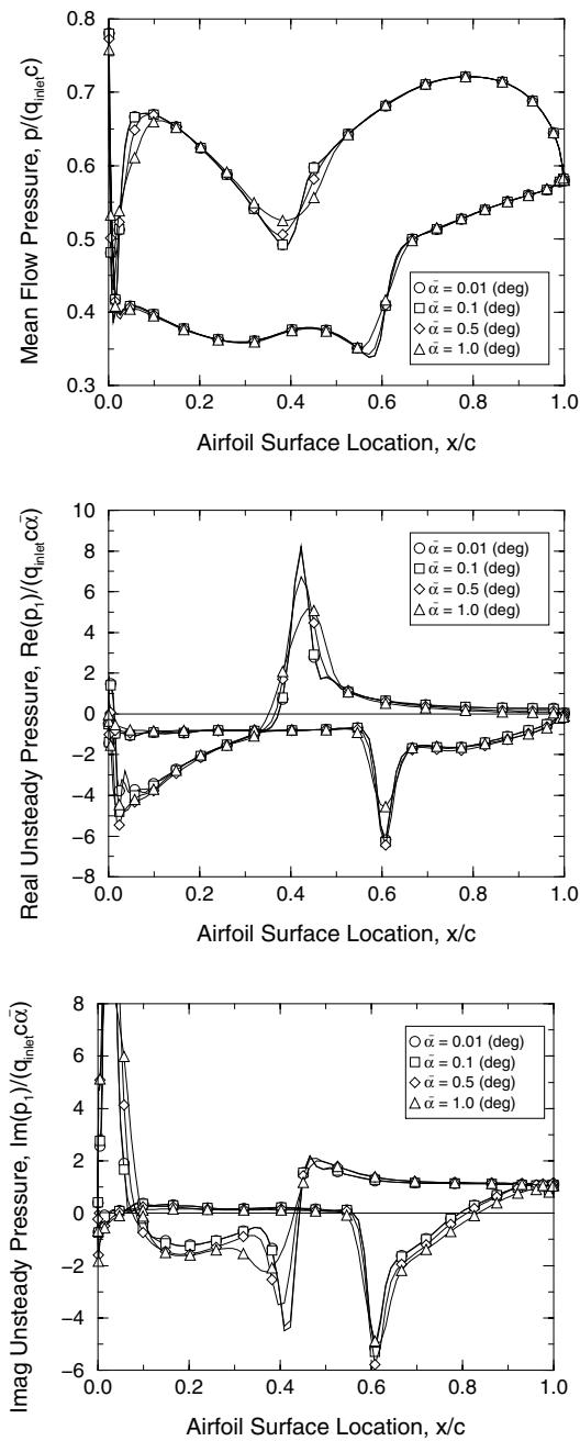
Figure 13.13. Unsteady pressure distribution for front stage compressor rotor airfoils vibrating in pitch with \bar{\omega} = 1.0 and \sigma = 30^\circ . Top: zeroth harmonic. Middle and bottom: first harmonic.
