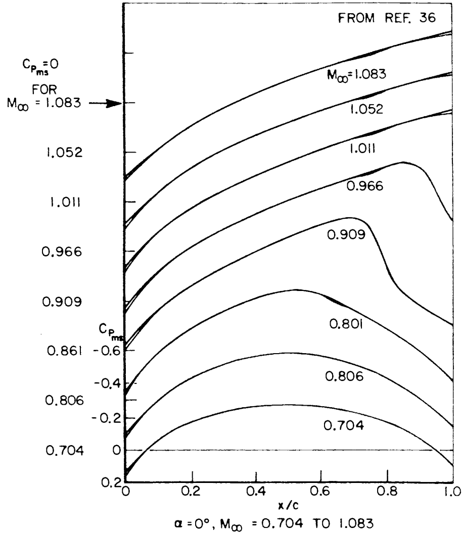
Figure 4.22. Representative experimental pressure distribution for 6-percent-thick circular-arc airfoil with roughness elements near the leading edge.
