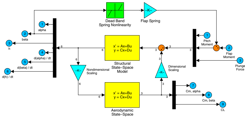
Figure 12.9. Coupled aeroelastic system with deadband nonlinearity
