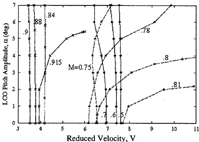
Figure 11.16. LCO Amplitude vs. Reduced Velocity for NACA 64A010 Airfoil
