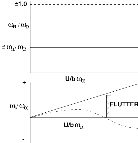
Figure 3.18. Real and imaginary components of frequency vs air speed.
