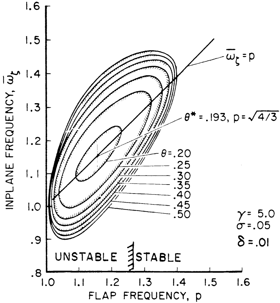
Figure 7.8. Flap lag stability boundaries. R = 0 , no elastic coupling [17].
