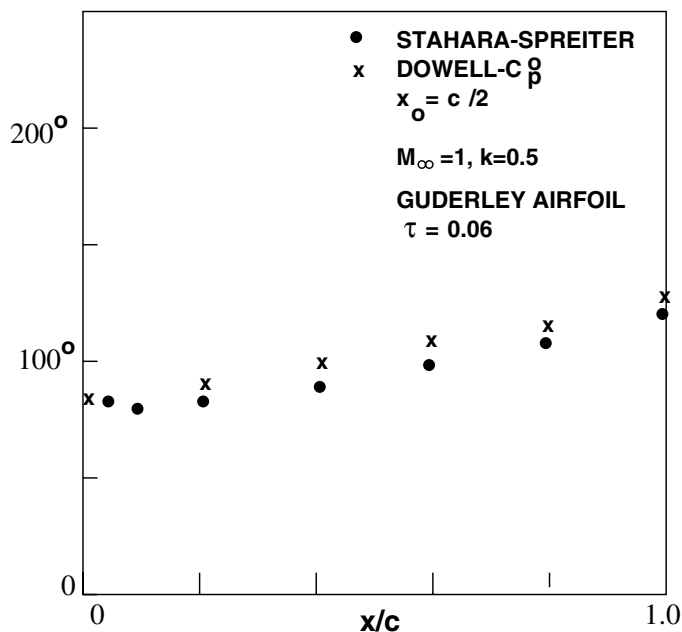
Figure 4.26. Pressure-translation phase angle distribution.
