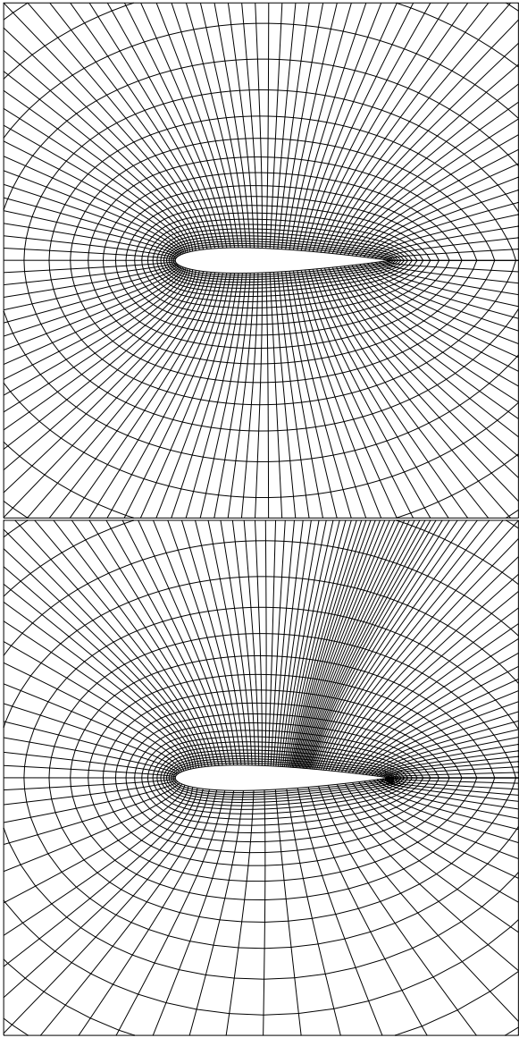
Figure 9.11. Typical 129 \times 43 -node grid about an NACA 0012 isolated airfoil. ( Top ) initial grid; ( bottom ) locally refined grid. (Republished from Florea et al (1999) with permission.)
