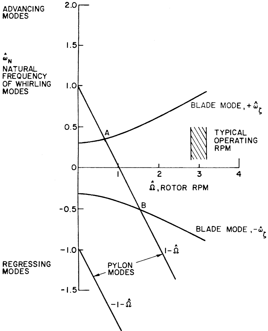
Figure 7.20. Uncoupled whirling modes ( \mu = 0 ). Rotating coordinate system.
