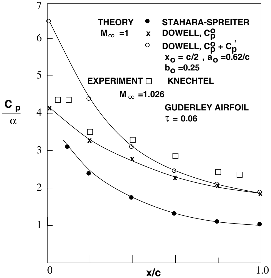
Figure 4.20. Pressure distribution for parabolic arc airfoil at constant angle of attack.
