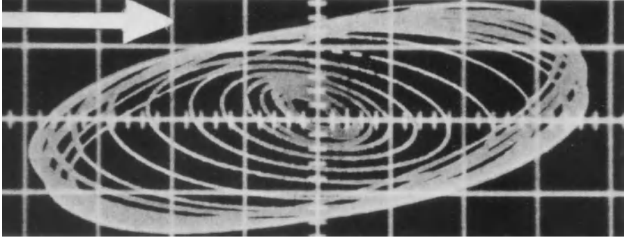
Figure 6.17. Amplitude trace of a wake galloping orbit (courtesy of National Aeronautical Establishment, National Research Council of Canada).
