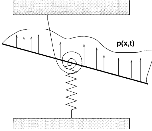
Figure 3.2. Typical section geometry.
