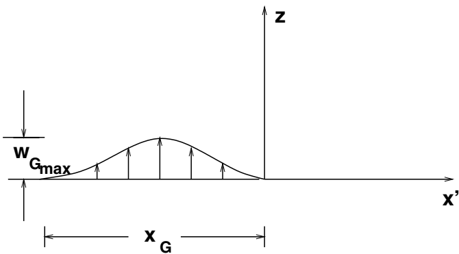
Figure 3.29. 1-COSINE gust.
