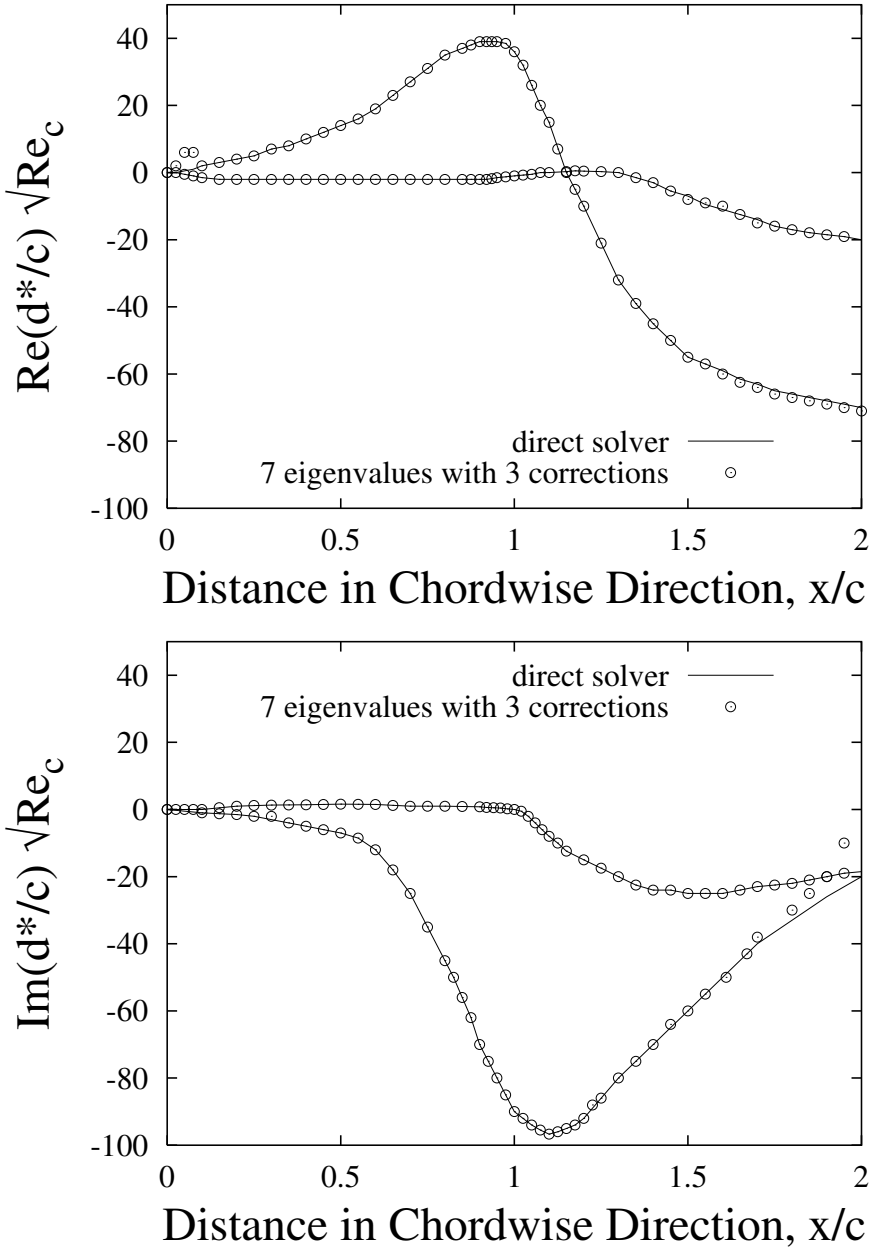
Figure 9.2. Real and imaginary (Im) parts of unsteady displacement thickness for airfoils pitching about a point near midchord. \Omega = 62^\circ ; \sigma = 90^\circ ; \bar{\omega} = 0.5 . (Republished from Florea et al (1996) with permission.)
