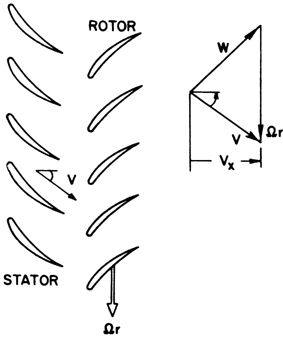
Figure 8.1. Velocity triangle in an axial compressor.
