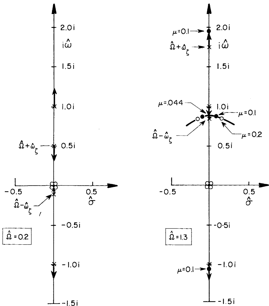
Figure 7.21. Root locus for increasing blade mass ratio ( \mu ) for two operating conditions.
