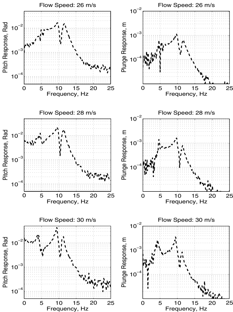
Figure 12.32. Closed loop transfer functions from spectral data with flap excitation.
