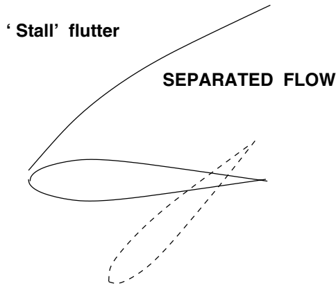
Figure 3.23. Schematic of separated flow geometry.
