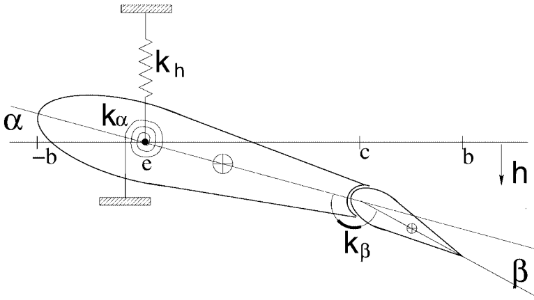
Figure 12.4. Typical section airfoil model
