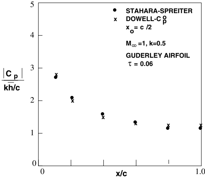
Figure 4.25. Pressure distribution for Guderley airfoil oscillating in rigid body translation.
