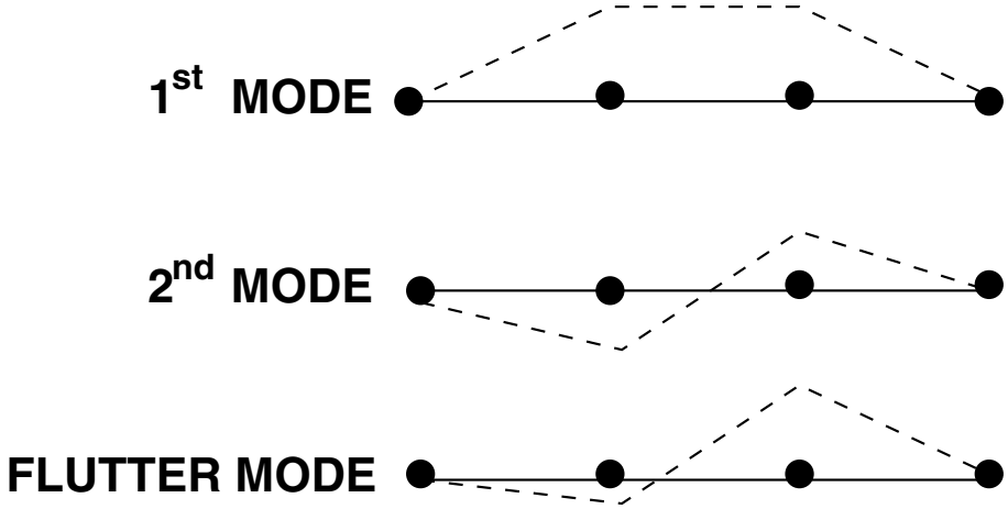
Figure 3.44. Natural modes and flutter mode
