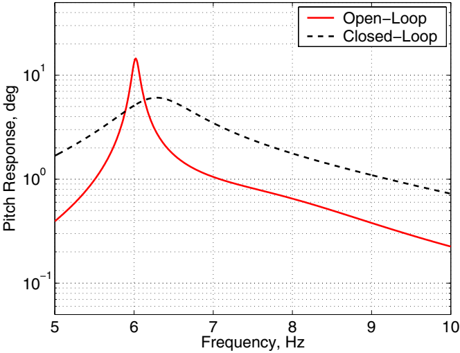
Figure 12.25. Open and Closed loop(LPV controller) gain from a force disturbance in plunge to motion in the pitch axes for the typical section model at U = 23 m/s near the open-loop flutter boundary of U_f = 23.4 m/s
