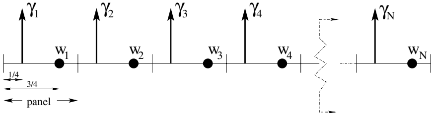
Figure 12.5. Arrangement of point vortices and control points for two dimensional vortex lattice aerodynamic model.
