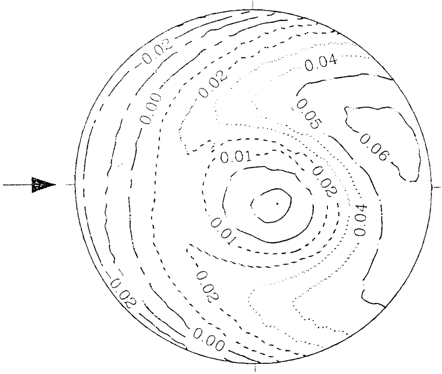
Figure 7.31. Theoretical induced inflow distribution, tapered, blades with fuselage, \mu = 0.15 , C_r = 0.0064 , \alpha = 3^\circ , M = 4 , S = 33 .
