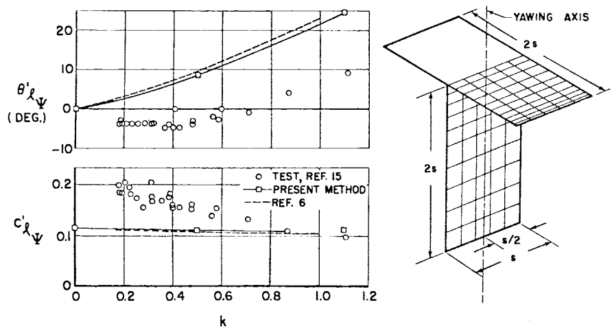
Figure 4.14. Rolling moment coefficient of horizontal stabilizer for simplified T-tail oscillating in yaw about fin mid-chord; simple harmonic motion.
