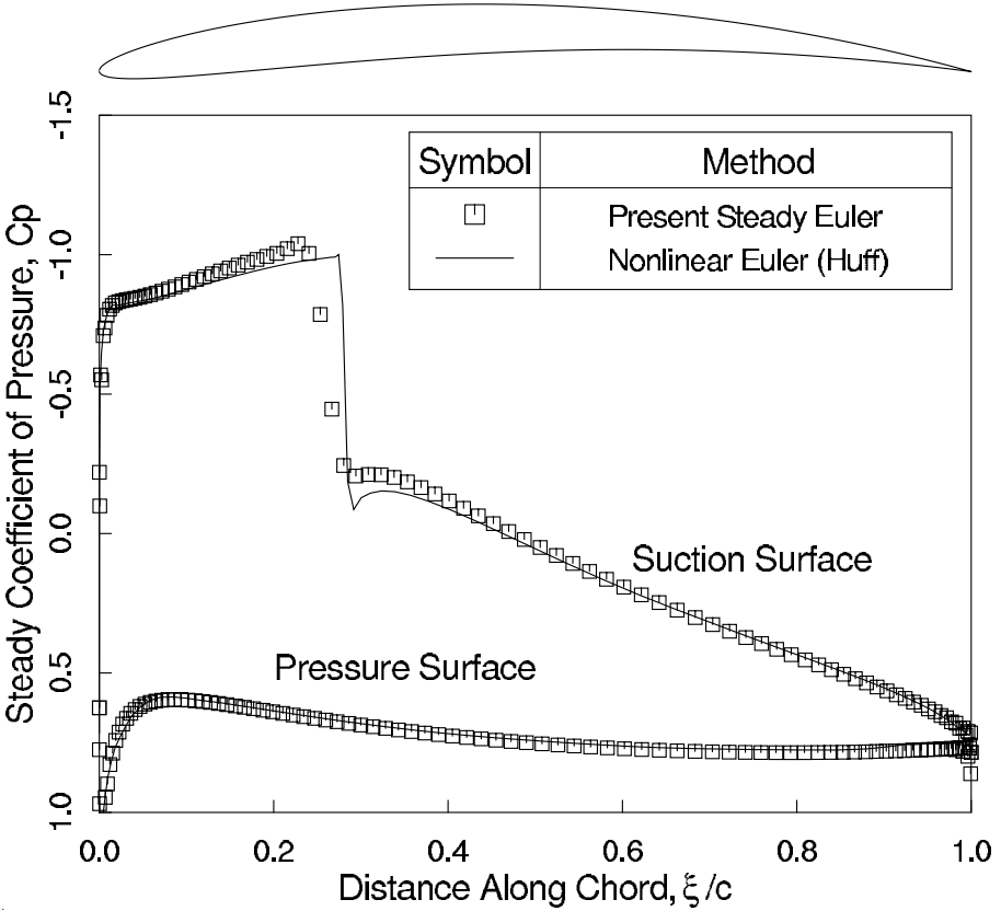
Figure 13.2. Steady surface pressure for the Tenth Standard Configuration transonic compressor cascade.
