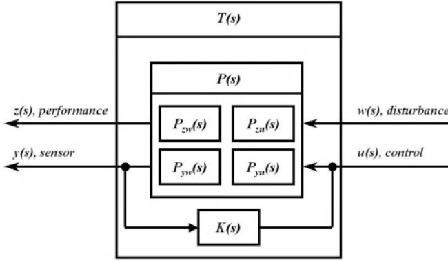
Figure 12.18. Block diagram of generalized plant with feedback controller.
