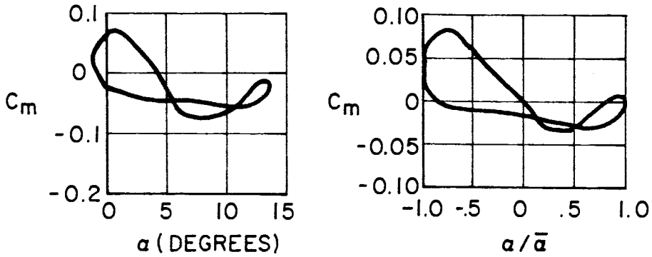
Figure 5.5. Dynamic moment loops.
