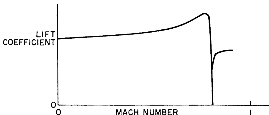
Figure 8.7. The aerodynamic resonance phenomenon.
