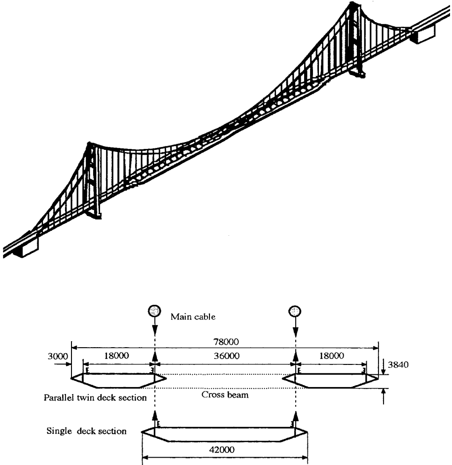
Figure 6.32. Spindle-type suspension bridge concept. From T. Miyata, “Comprehensive Discussions on Aeroelastic-Coupled Flutter Control for Very Long Suspension Bridges,” in Long-Span Bridges and Aerodynamics , Springer-Verlag, Berlin (1999), 181-200.
