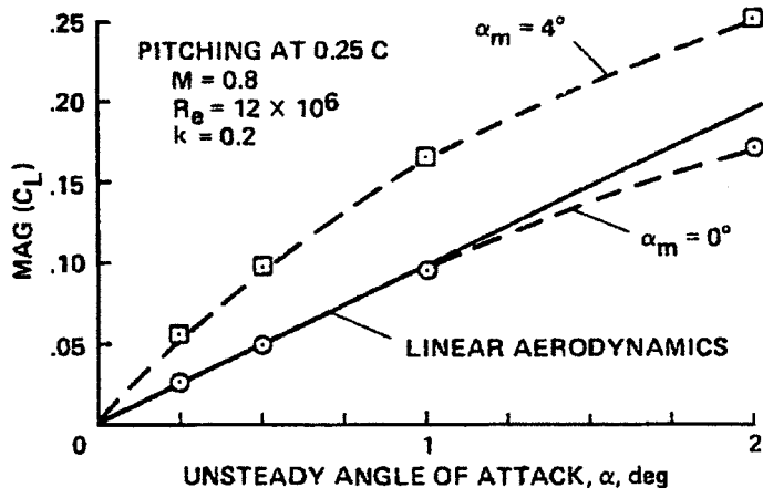
Figure 11.5. Unsteady Lift Magnitude vs. Unsteady Angle of Attack Magnitude
