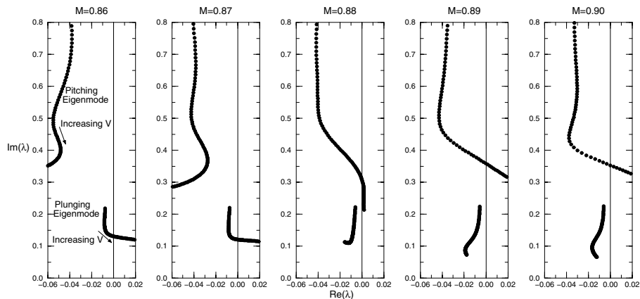
Figure 9.10. Loci of pitching and plunging roots of aeroelastic system. \text{Re}(\lambda) , real eigenvalues; \text{Im}(\lambda) , imaginary eigenvalues; M , Mach number; V , variation. (Republished from Hall et al (1999) with permission.)
