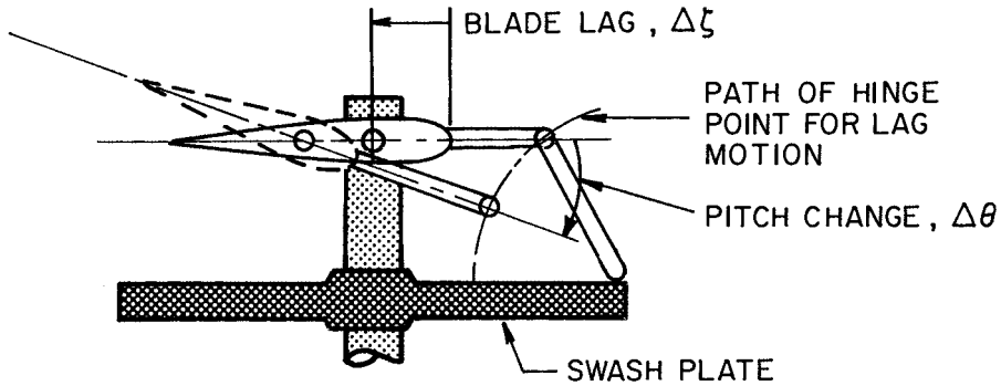
Figure 7.4. Pitch-lag coupling due to pitch link geometry. Articulated rotor.
