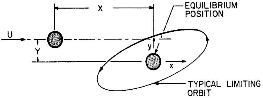
Figure 6.18. Coordinates for wake galloping analysis [43].
