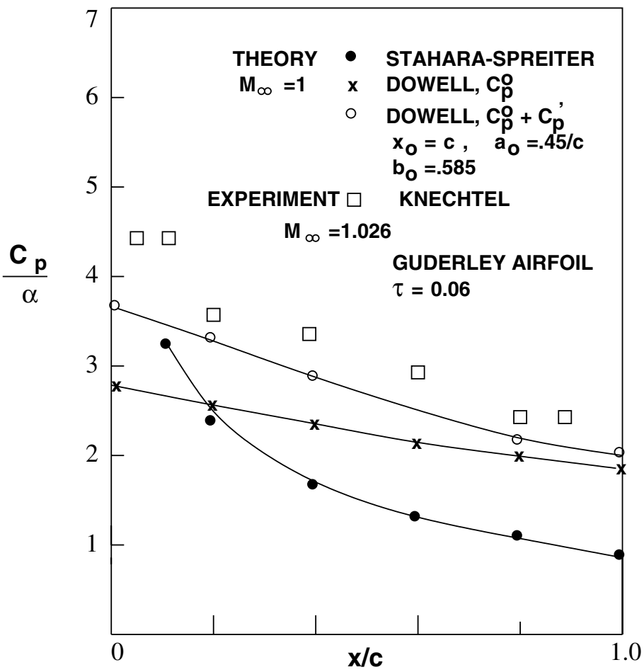
Figure 4.21. Pressure distribution for parabolic arc airfoil at constant angle of attack.
