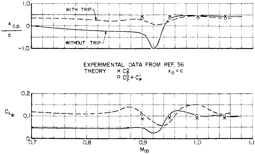
Figure 4.24. Effects of boundary-layer trip in the variation with Mach number of lift-curve slope and center pressure of the circular-arc airfoil at \alpha_o \simeq 0^\circ .
