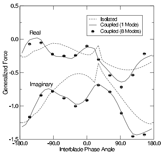
Figure 13.9. Generalized force acting on rotor blades vibrating in first bending.
