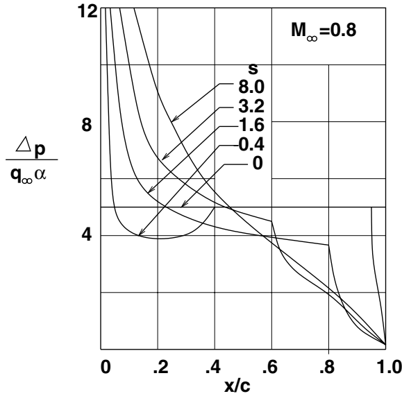
Figure 4.9. Chordwise lifting pressure distributions.
