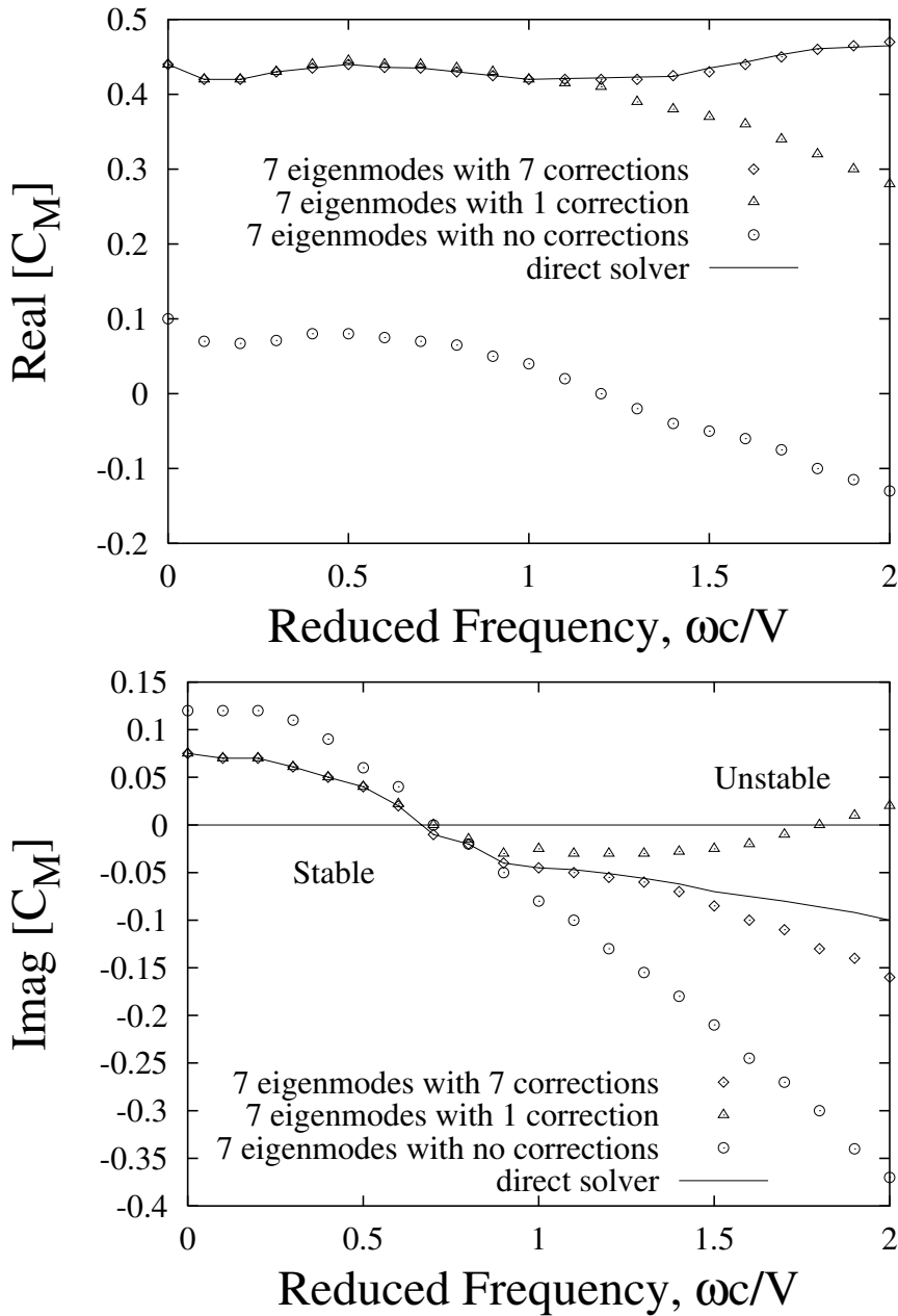
Figure 9.1. Real and imaginary (Imag) pitching moment for airfoils pitching about a point near midchord for a range of reduced frequencies . \Omega = 62^0 ; \sigma = 90^0 . (Republished from Florea et al (1996) with permission.)
