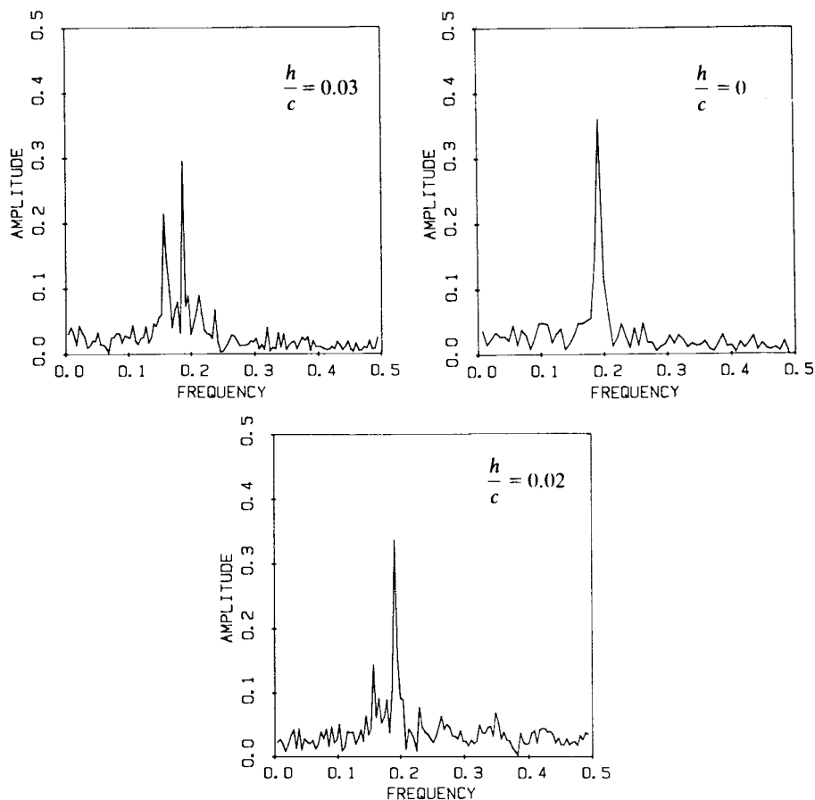
Figure 5.7. Effect of vibration amplitude on lift amplitude and frequency.
