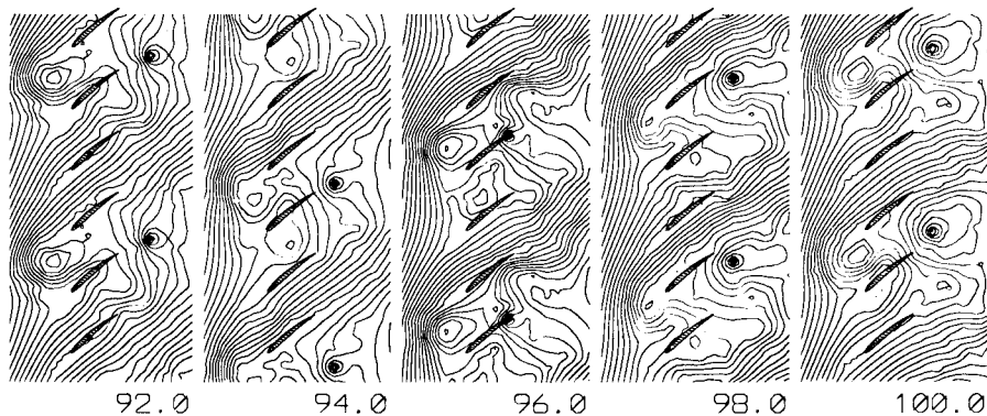
Figure 5.6. Streamline pattern at several instants for bending vibrations in stall.
