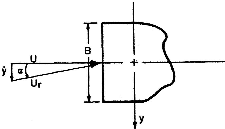
Figure 6.9. Effective angle of attack on an oscillating bluff object.
