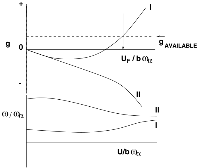
Figure 3.20. Structural damping and frequency required for neutrally stable motion vs air speed.
