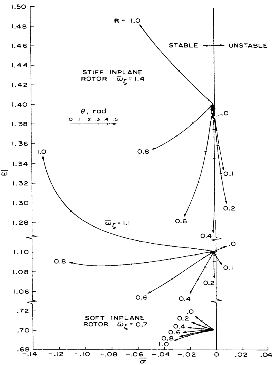
Figure 7.10. Locus of roots for increasing blade pitch with various levels of elastic coupling [17].
