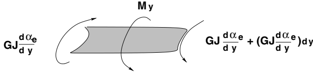
Figure 2.8. Differential element of beam-rod.
