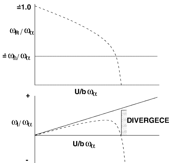
Figure 3.19. Real and imaginary components of frequency vs air speed
