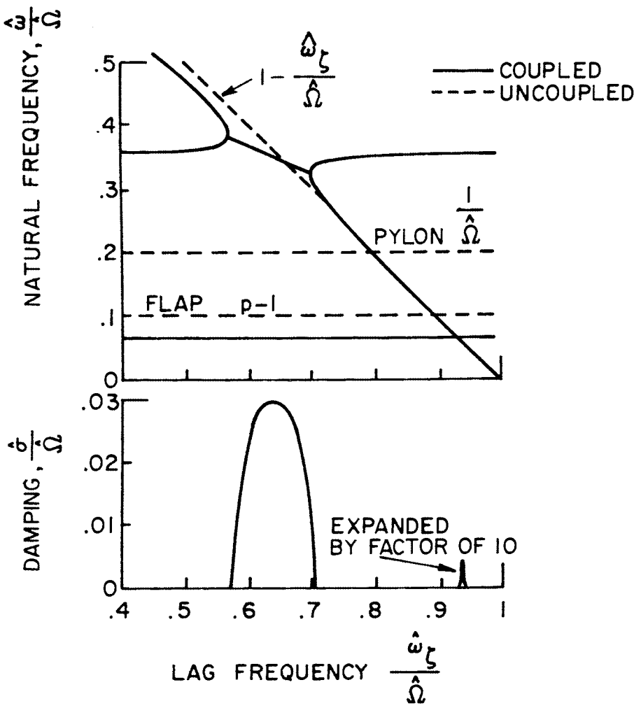
Figure 7.26. Frequency and damping of rotor-body system. Flap, lag and pylon pitch degrees of freedom. No aerodynamics [10].
