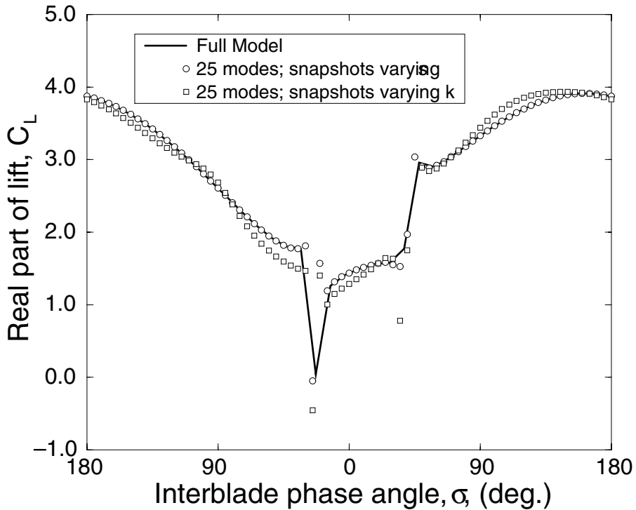
Figure 9.19. Real part of the coefficient of lift C_L obtained by using 25 POD modes when the reduced frequency k is 0.85, and the upwind far-field Mach number M is 0.5. (Republished with permission from Epureanu et al (2001).)
