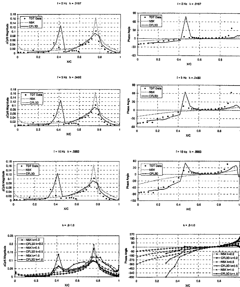
Figure 11.3. Unsteady Pressure Distribution of BACT Model
