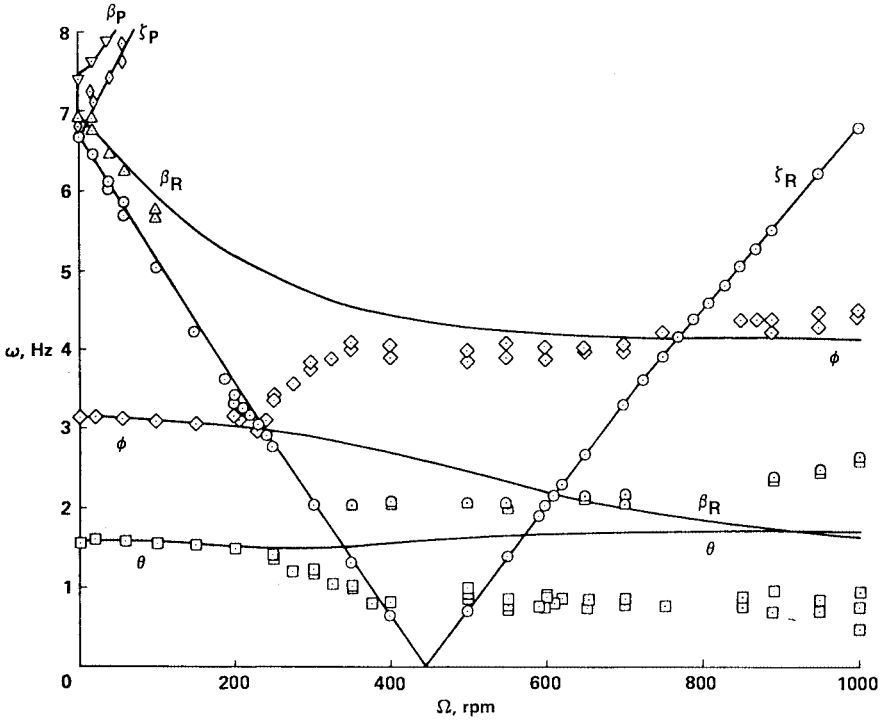
Figure 7.28. Influence of unsteady aerodynamics on hingeless rotor ground resonance. Comparison of measured modal frequencies, and calculations without dynamic inflow.
