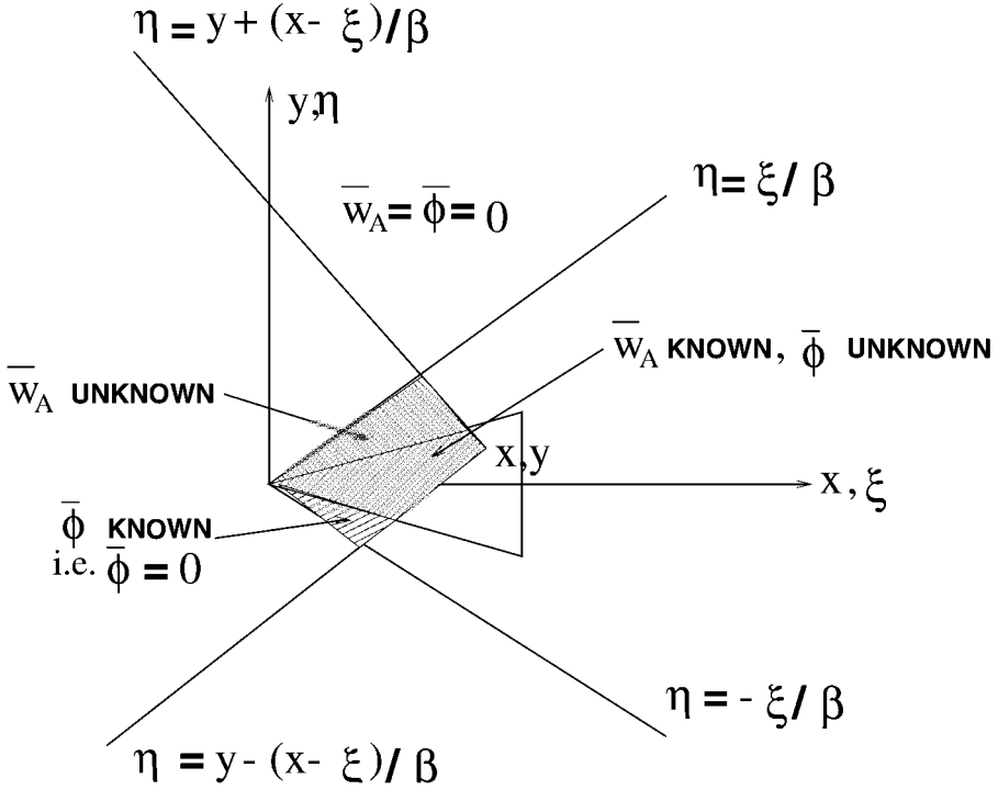
Figure 4.4. Lifting surface geometry. A representative delta wing is shown.
