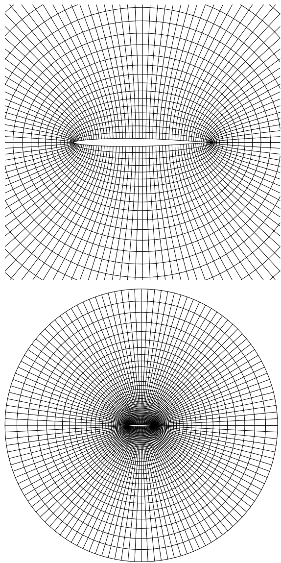
Figure 9.7. Computational grid used for an NACA 64A006 airfoil. (Republished from Hall et al (1999) with permission.)
