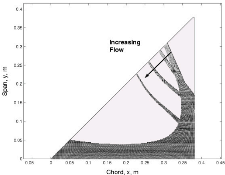
Figure 12.17. Mode shape progression of second aeroelastic mode with flow speed.
