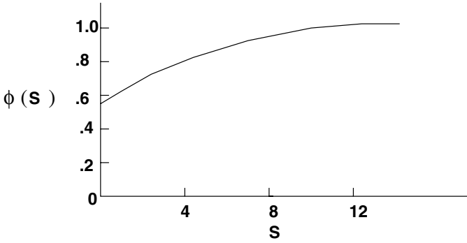
Figure 3.7. Wagner function.
