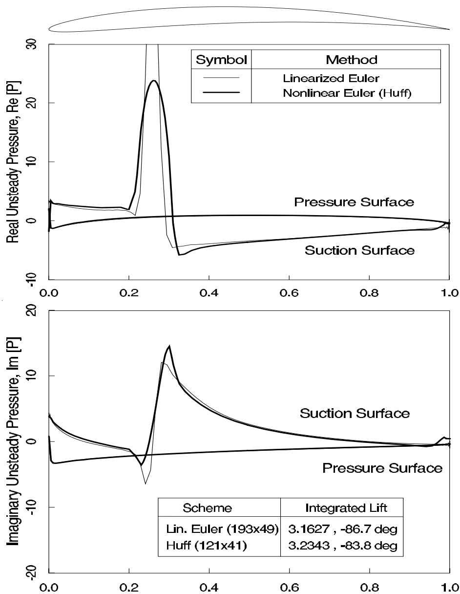
Figure 13.3. Real and imaginary surface pressure for the Tenth Standard Configuration cascade vibrating in plunge with a reduced frequency \overline{\omega} of 1.287 with an interblade phase angle \sigma of -90 deg.
