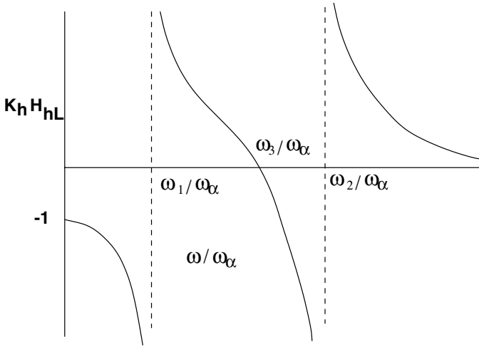
Figure 3.3. Transfer function.
