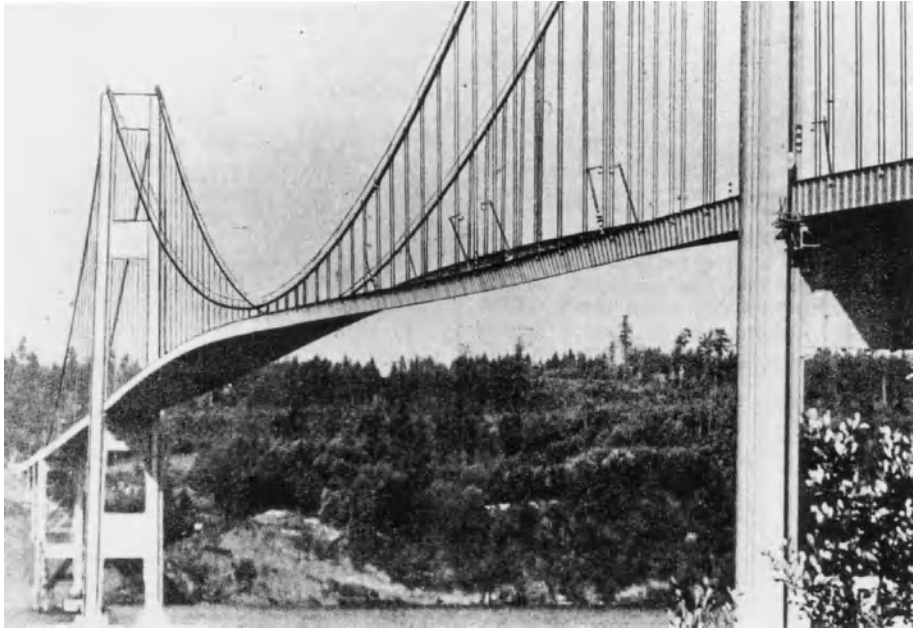
Figure 6.2. Flutter of the Tacoma Narrows Bridge, November 10, 1940. From F.B. Farquharson (ed.), Aerodynamic Stability of Suspension Bridges , 1949-1954.
