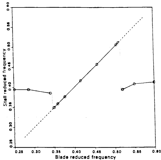
Figure 5.8. Influence of blade-reduced frequency on the stall-reduced frequency for a cascade in torsional vibration. The plot shows the entrainment of stall frequency on a certain interval of blade frequency.
