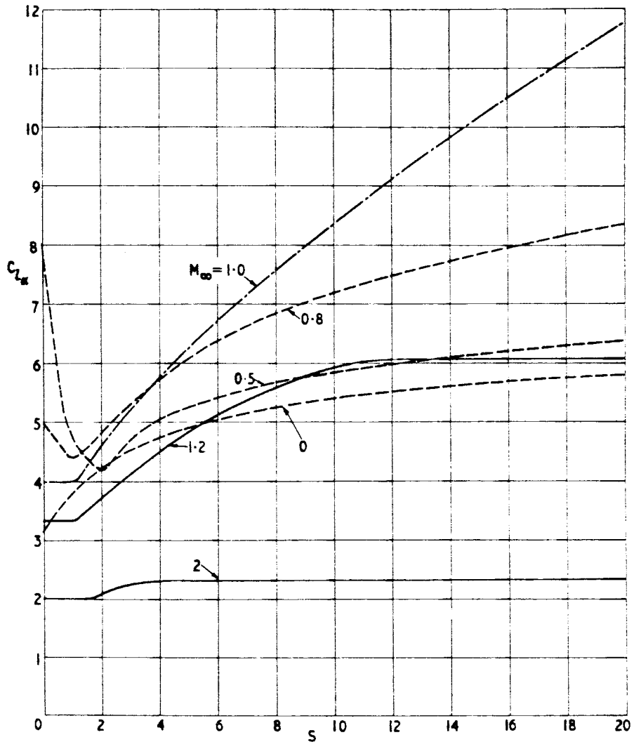
Figure 4.11. Time history of lift curve slope.
