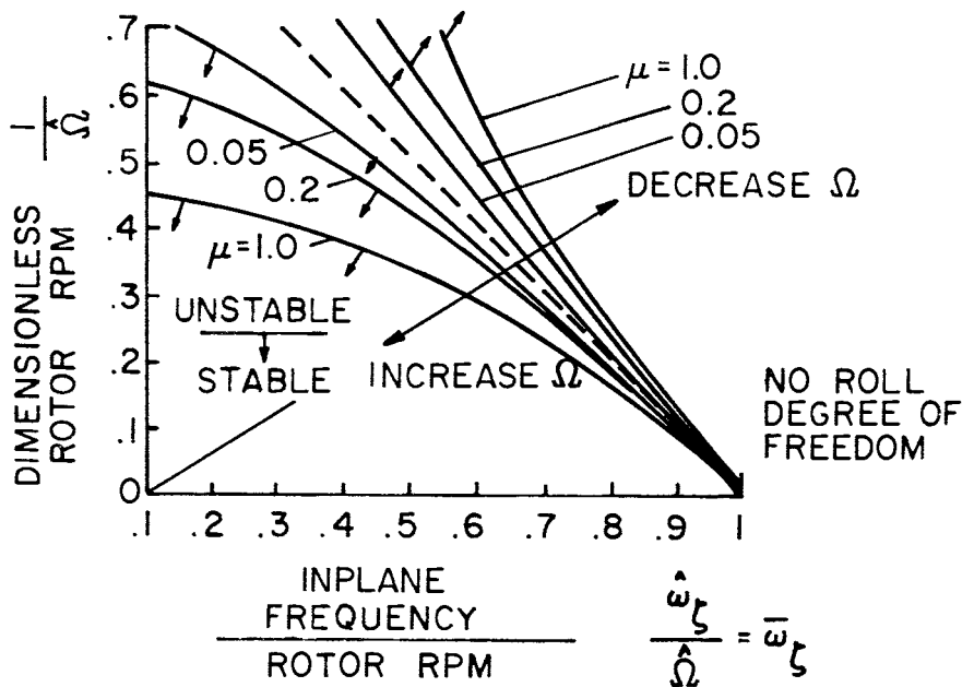
Figure 7.22. Extent of unstable region for various mass ratios.
