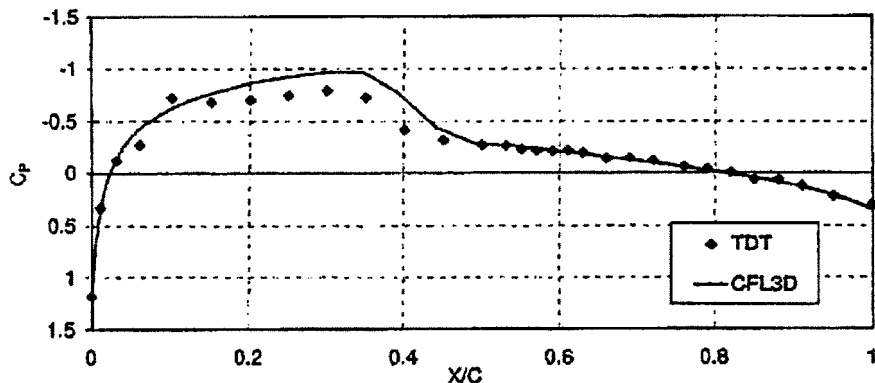
Figure 11.2. Steady State Pressure Distribution for BACT Model
