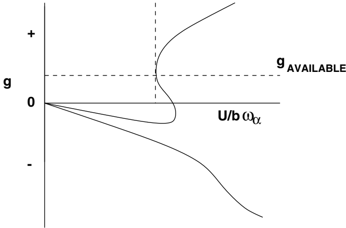
Figure 3.21. Structural damping required for flutter vs air speed.
