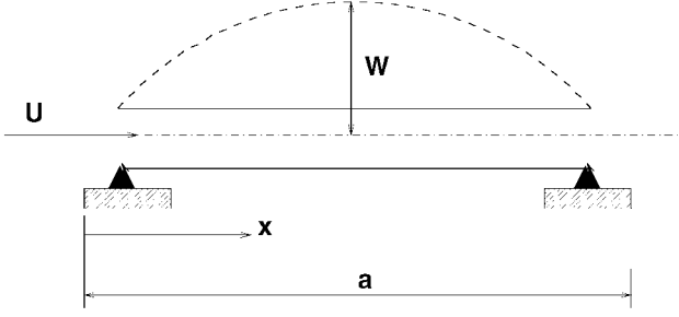
Figure 2.15. Fluid flow through a flexible pipe.
