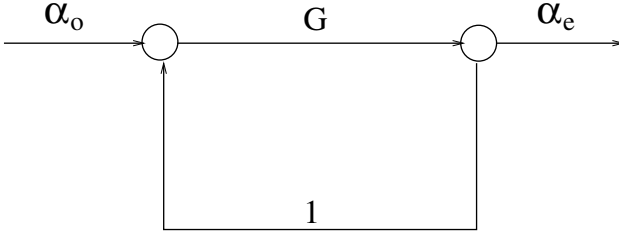
Figure 2.3. Feedback representation of aeroelastic divergence.
