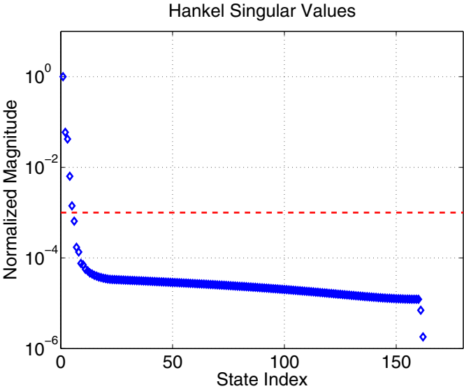
Figure 12.6. Hankel singular values for balanced realization of flat-plate aerodynamic model
