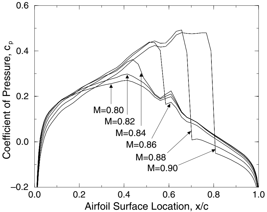
Figure 9.8. Steady-background-flow surface pressure coefficient. M , Mach number. (Republished from Hall et al (1999) with permission.)
