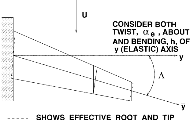
Figure 2.17. Sweptwing geometry.
