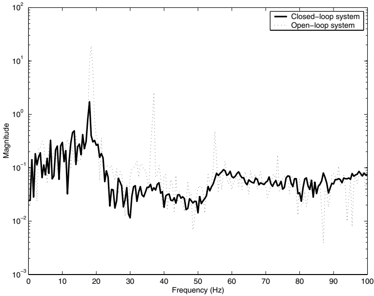
Figure 12.35. Comparison of open-loop and closed-loop system, configuration Case 1 at 37.5 m/s
