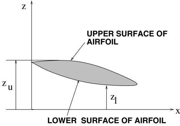
Figure 4.2. Airfoil geometry.
