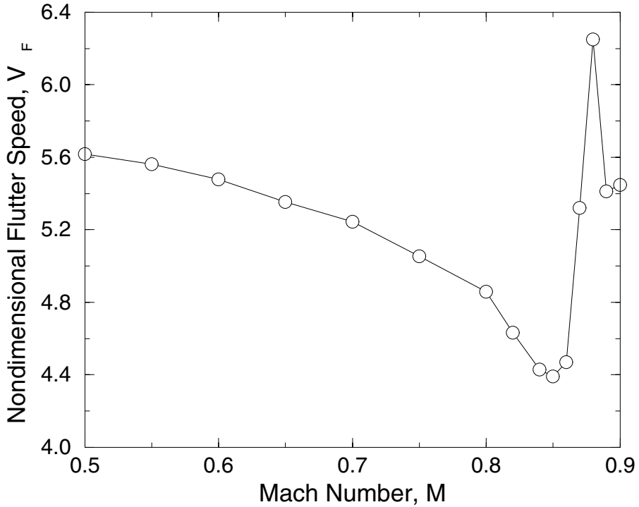
Figure 9.9. Flutter speed variation ( V_F ) with Mach number ( M ). (Republished from Hall et al (1999) with permission.)
