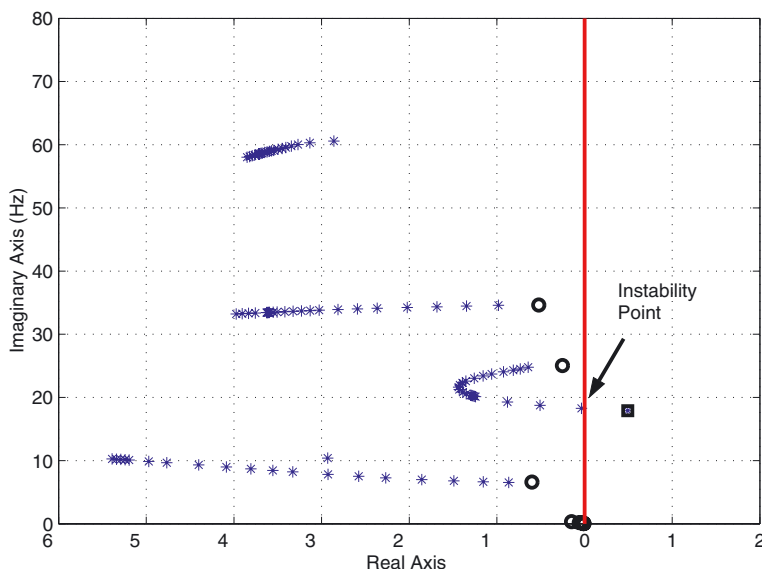
Figure 12.16. Aeroelastic root migrations with flow.
