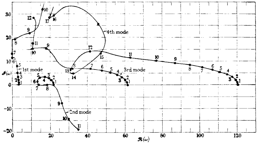
Figure 3.40b. The dimensionless complex frequency of the four lowest modes of the system as a function of the dimensionless flow velocity for \beta = 0.295 .
