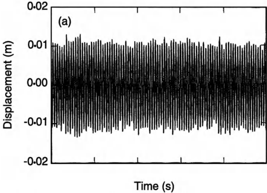
Figure 6.15. Observed time history of displacement y .
