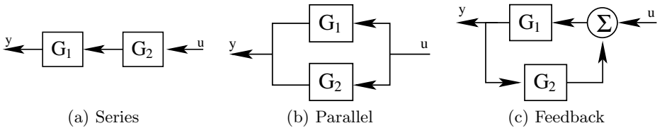
Figure 12.1. Interconnection of systems G_1 and G_2
