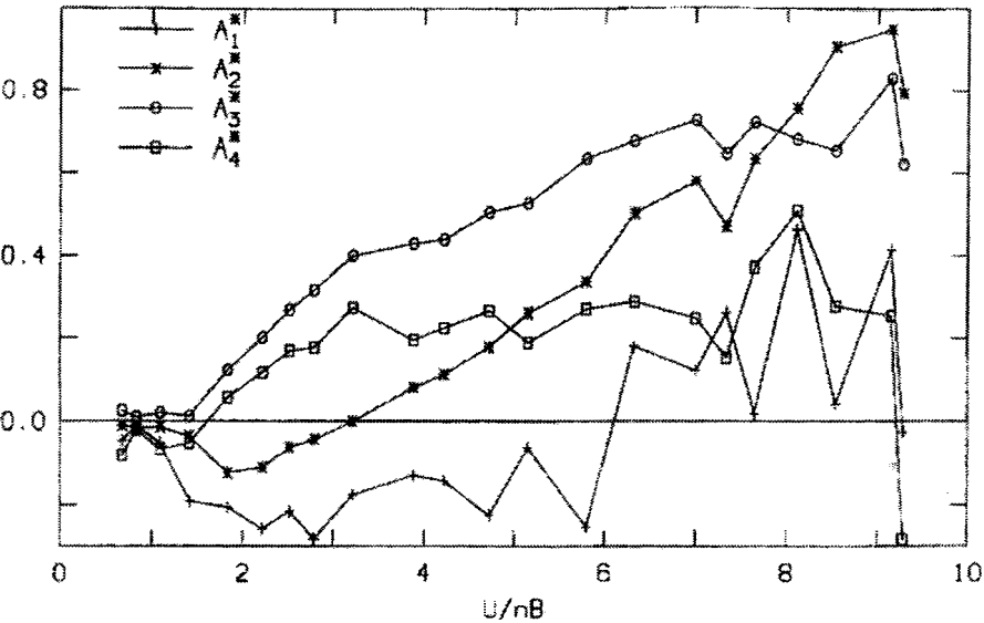
Figure 6.27. A_i^* flutter derivatives of Golden Gate bridge at 0^\circ ( i = 1, 2, 3, 4 ).
