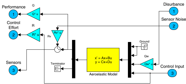
Figure 12.20. Block diagram showing system augmentation for H_2 control design problem
