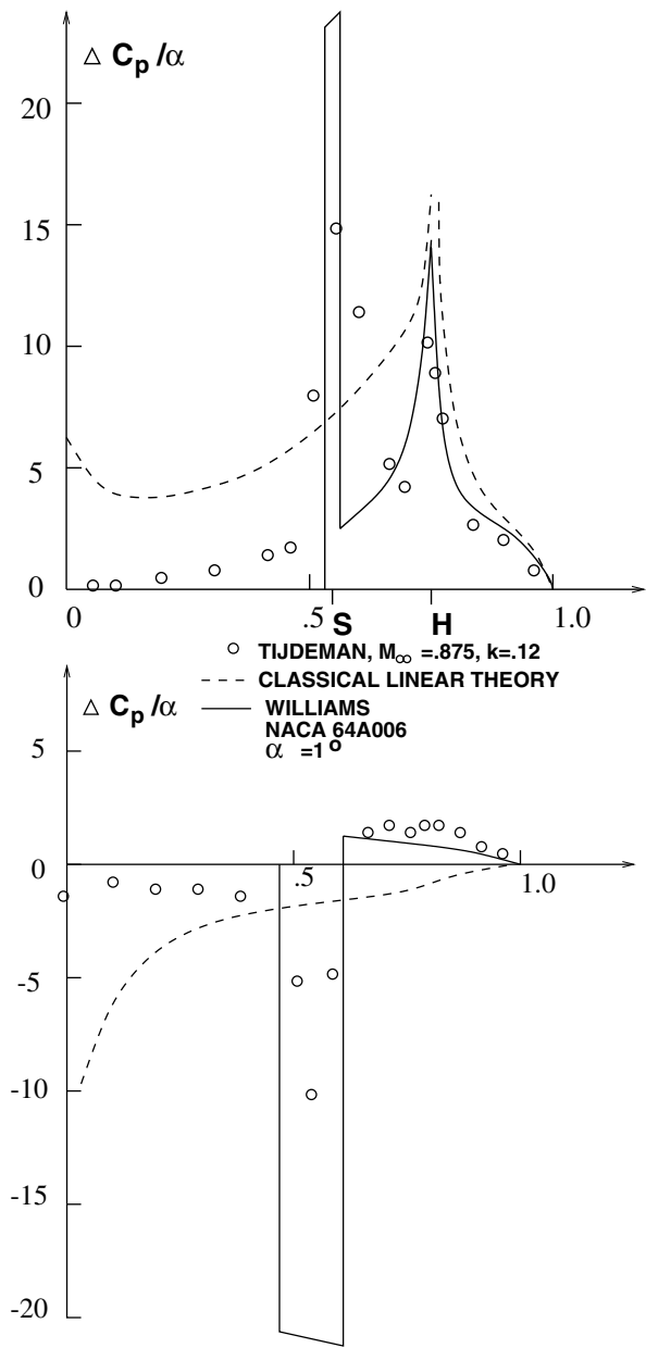
Figure 4.27. (a)(top) In phase pressure, and (b) (bottom) out of phase pressure
