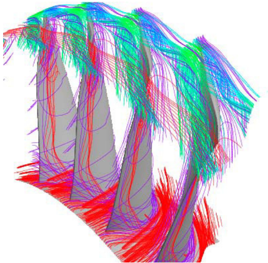
Figure 13.4. Computed steady streamline patterns for a modern front stage compressor rotor.
