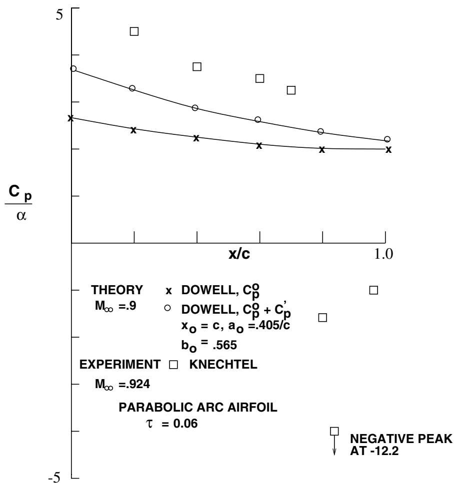
Figure 4.23. Pressure distribution for parabolic arc airfoil at constant angle of attack.
