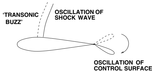
Figure 3.22. Schematic of transonic buzz geometry.
