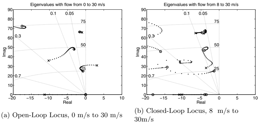
Figure 12.27. Root Locus of (a) open-loop identified LPV model, with a flutter prediction at 26.8 m/s. In (b), predicted closed-loop locus with LPV design and constraint of 5% damping.
