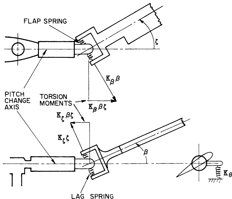
Figure 7.11. Simplified blade model for flap-lag-torsion coupling.
