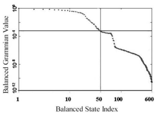
Figure 12.15. Relative magnitude of Gramians in balanced system.
