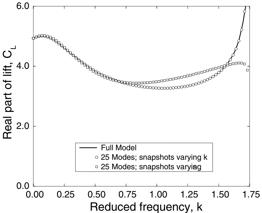
Figure 9.20. Real part of the coefficient of lift C_L obtained by using 25 POD modes when the interblade phase angle \sigma is 90^\circ and the upwind far-field Mach number M is 0.5. (Republished with permission from Epureanu et al (2001).)
