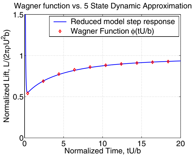
Figure 12.7. Comparison of the Wagner function and step response of reduced order aerodynamics model
