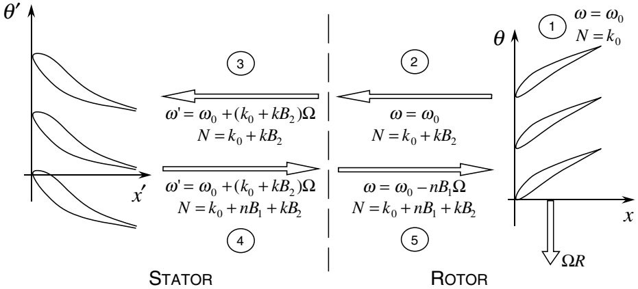
Figure 13.6. Kinematics of mode scattering and frequency shifting in a multistage machine.
