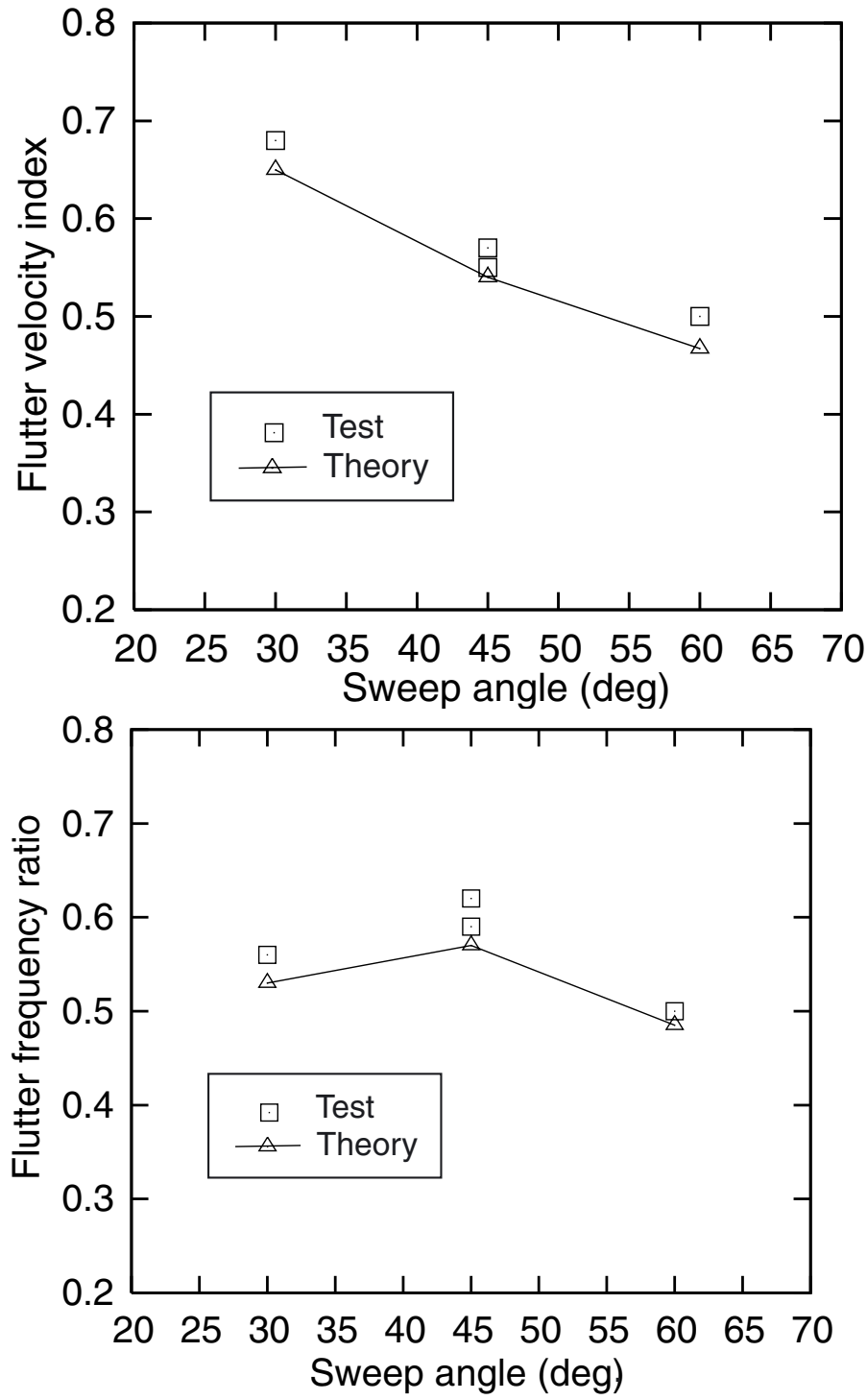
Figure 9.22. Variation of flutter velocity index (top) and flutter frequency ratio (bottom) with sweep angle. (Republished with permission from Tang et al (1999).)
