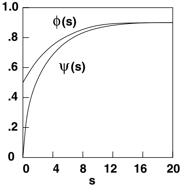
Figure 4.7. Wagner's function \phi(s) for indicial lift and Küssner's function \psi(s) for lift due to a sharp-edged gust, plotted as functions of distance travelled in semi-chordlengths. After BAH, Fig 5.21.
