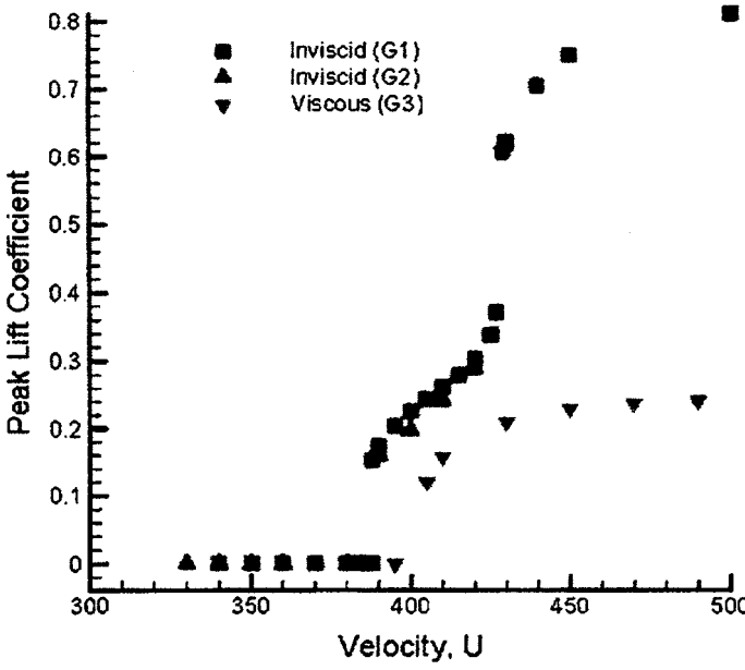
Figure 11.25. LCO Response vs. Flow Velocity for Goland Wing
