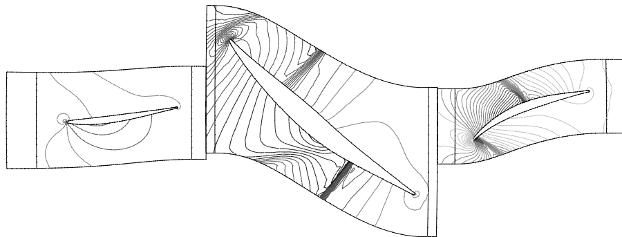
Figure 13.7. Pressure contours at the midspan of a front stage compressor.
