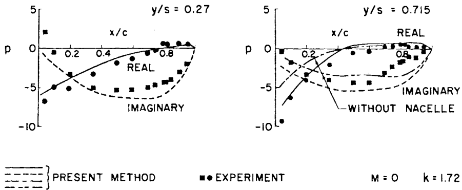
Figure 4.17. Comparison of experimental and calculated lifting pressure coefficient on a wing-nacelle combination oscillating in pitch; simple harmonic motion.
