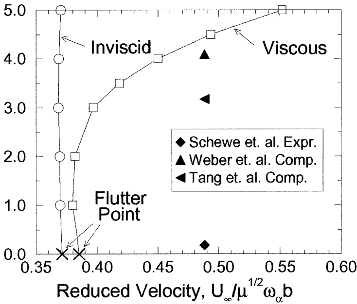
Figure 11.17. LCO Amplitude vs. Reduced velocity for NCR 7301 Supercritical Airfoil
