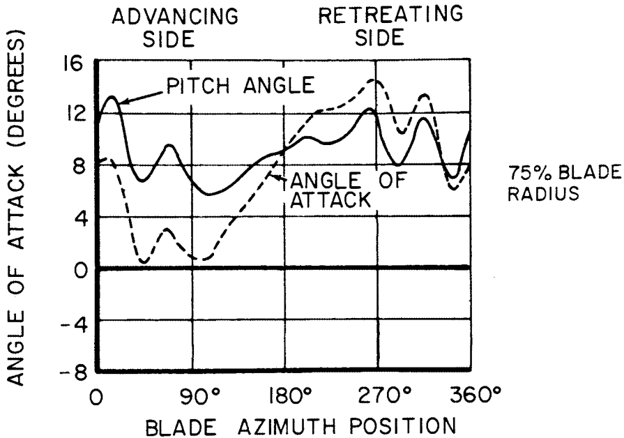
Figure 7.15. Typical time history of blade motion for blade encountering stall flutter [42].
