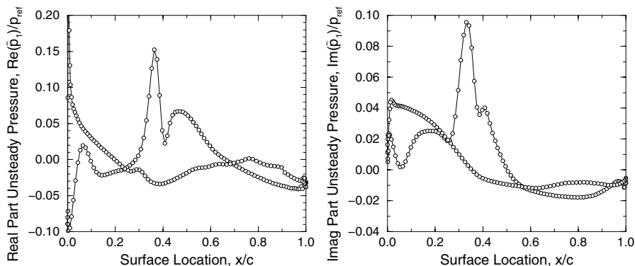
Figure 13.5. Unsteady pressure distribution near the midspan station of a front stage compressor rotor. The airfoil vibrates in its first bending mode with an interblade phase angle of zero.
