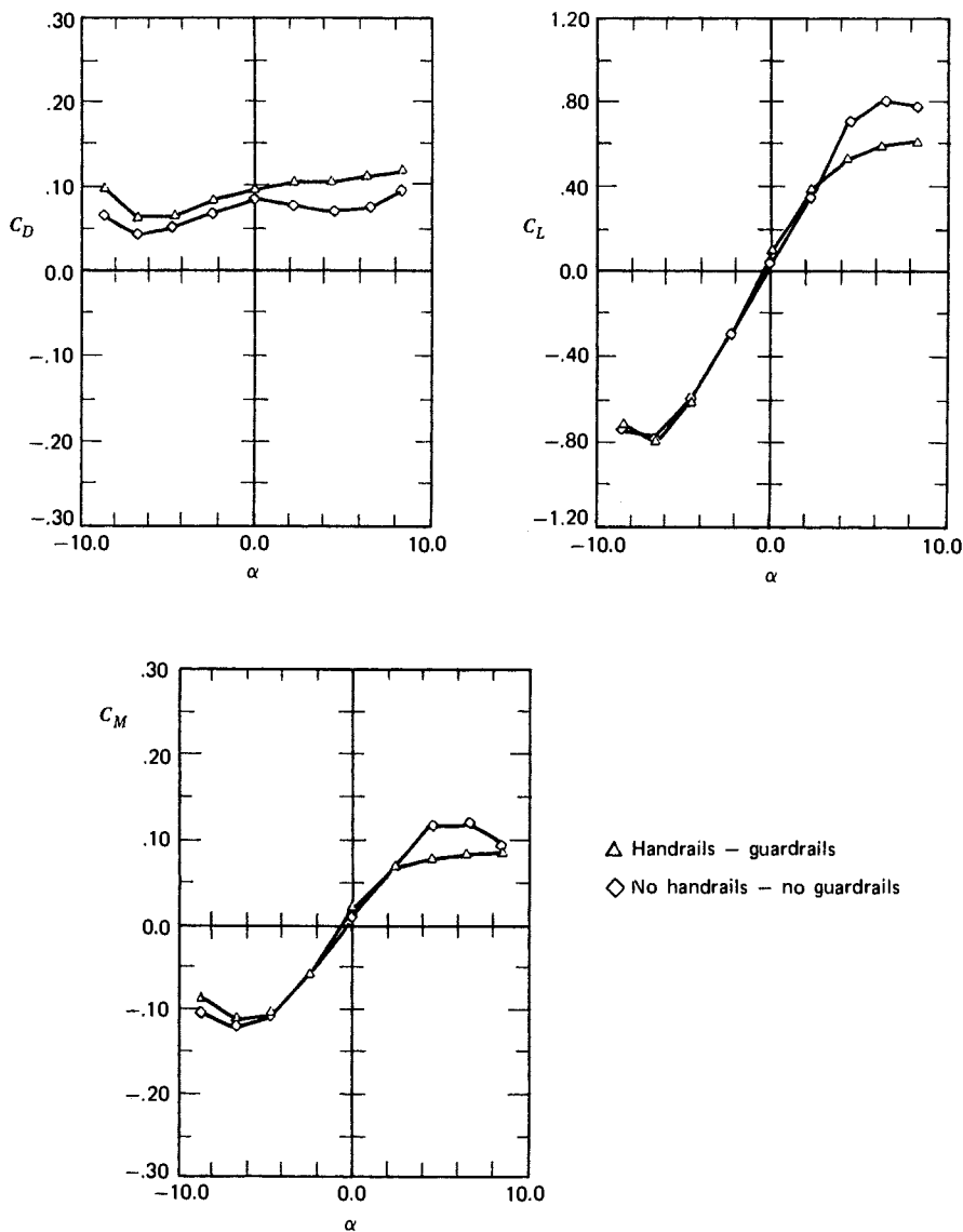
Figure 6.25. Drag, lift, and aerodynamic coefficients for proposed deck of New Burrard Inlet Crossing [61] (courtesy of the National Aeronautical Establishment, National Research Council of Canada).
