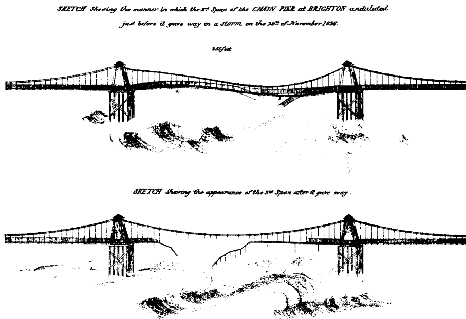
Figure 6.1. Brighton Chain Pier Bridge failure, Nov. 29, 1836, as sketched by W. Reed. From J.S. Russell, "On the Vibration of Suspension Bridges and Other Structures, and the Means of Preventing Injury from this Cause," Trans. Royal Scottish Soc. Arts (1841), quoted in F.B. Farquharson (ed.), Aerodynamic Stability of Suspension Bridges , Bulletin No. 116, University of Washington Engineering Experiment Station, Seattle, 1949-1954.
