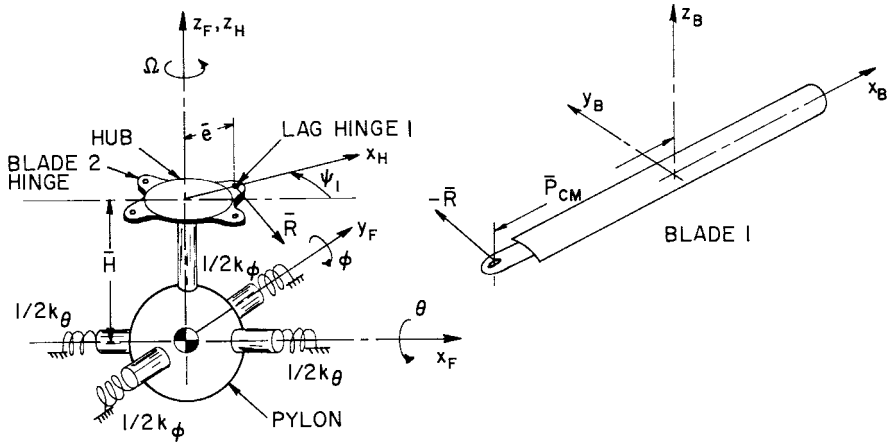
Figure 7.18. Free body diagram for ground resonance analysis.
