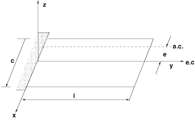
Figure 2.7. Beam-rod representation of wing.
