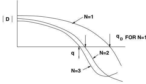
Figure 2.11. Characteristic determinant vs dynamic pressure.
