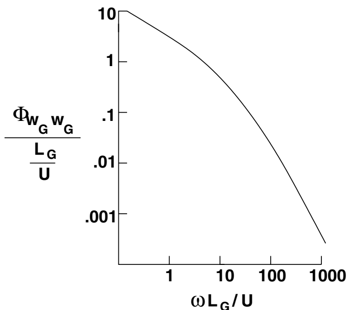
Figure 3.31. Gust power spectral density.
