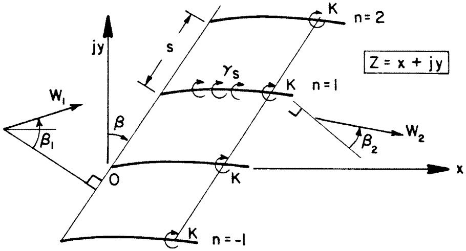
Figure 8.6. Cascade camberlines modelled by vortex sheets.
