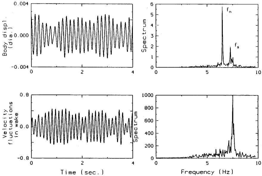
Figure 6.5c. Response for U/f_n D = 5.475 ; \zeta = 0.15\% .
