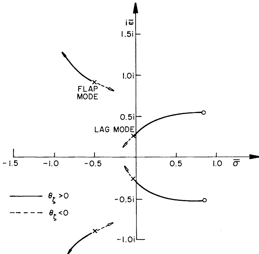
Figure 7.5. Effect of pitch-lag coupling on flap-lag stability.
