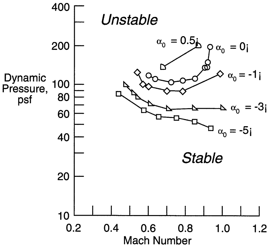
Figure 11.7. Flutter Dynamic Pressure vs. Mach Number for Various Mean Angles of Attack
