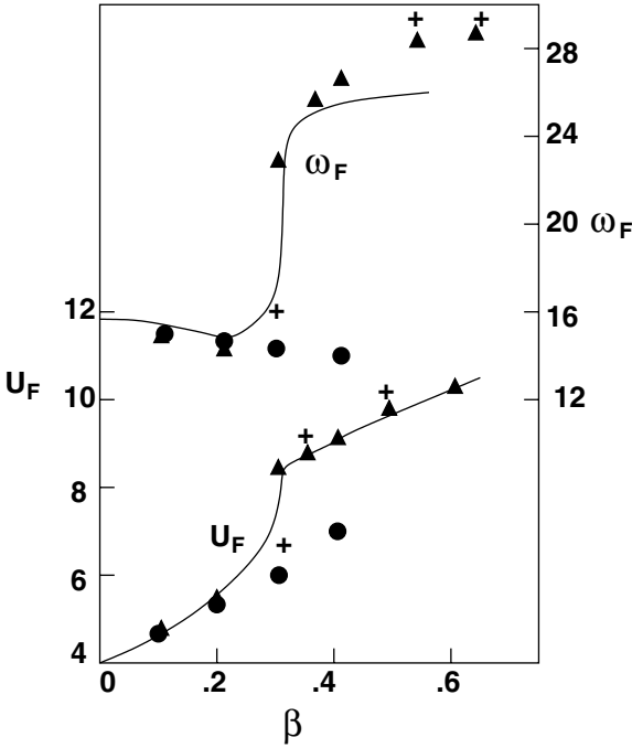
Figure 3.41. Flutter boundary for flexible pipe
