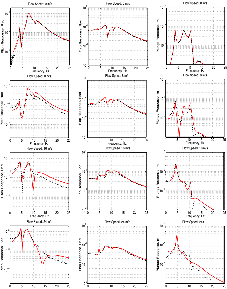
Figure 12.29. Comparison of LPV model obtained through tuned aeroelastic coupling (solid) and transfer functions based on spectra from experimental data (dashed).
