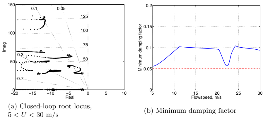
Figure 12.24. Root Loci as flowspeed is varied from 5 m/s (Circle) to 30 m/s (X) with gain-scheduled LPV control law. Closed-loop system retains minimum of 5% damping through the design range.
