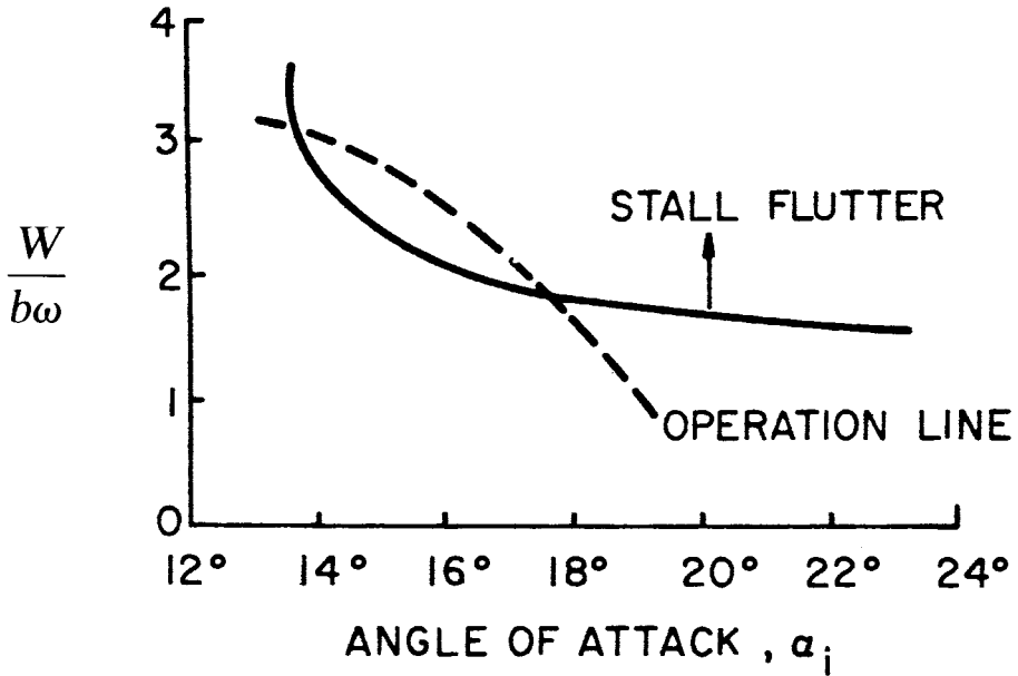
Figure 8.9. Experimental stall flutter correlation.
