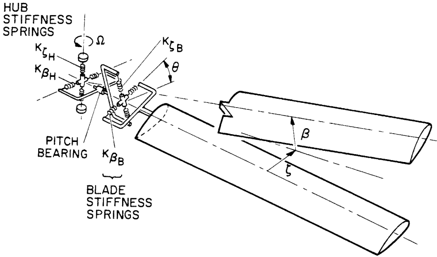
Figure 7.6. Spring model for elastic blade and hub.
