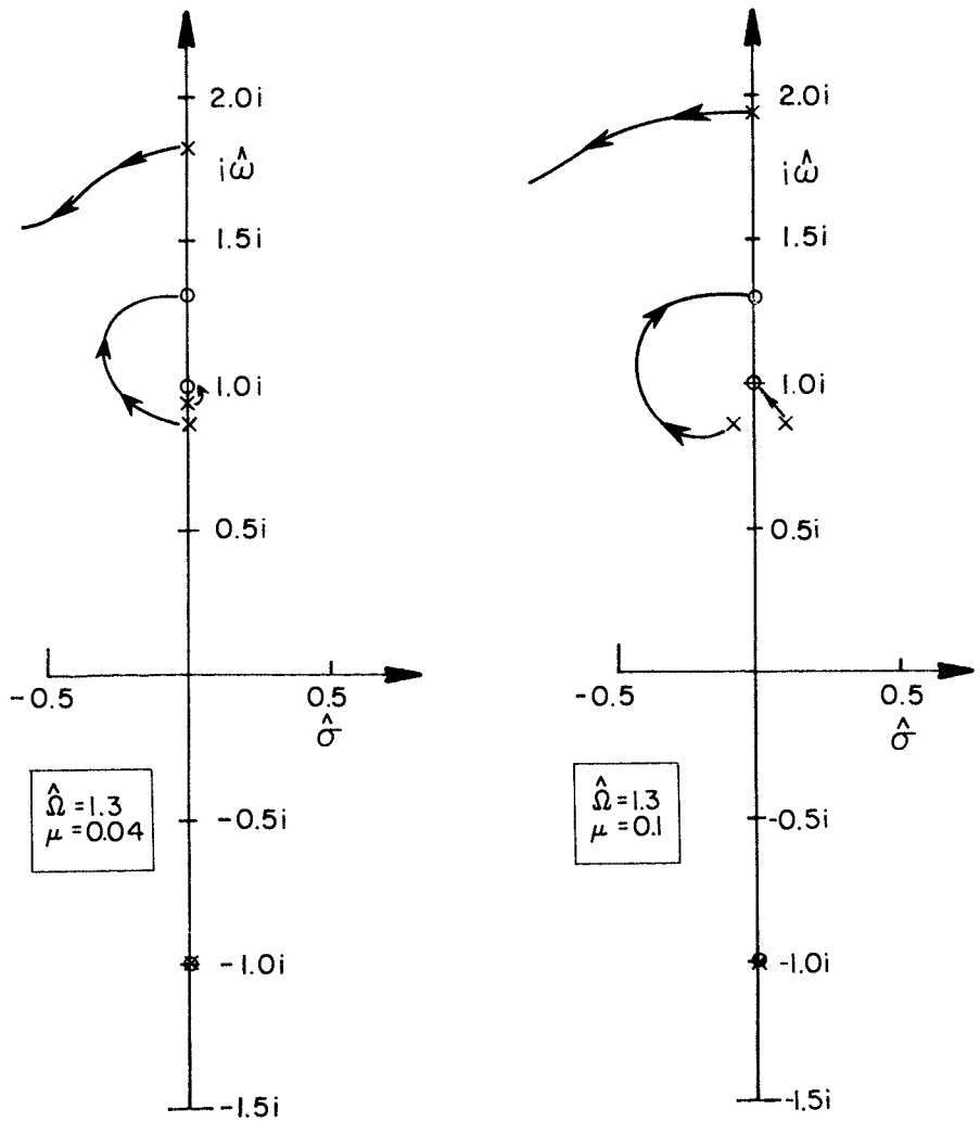
Figure 7.24. Root locus for increasing lag (rotating axis) damping on ground resonance stability.
