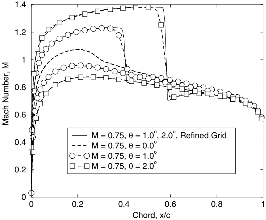
Figure 9.12. Steady Mach number ( M ) and pressure distribution on surface of NACA 0012 airfoil at different angles of attack. Freestream Mach number M_\infty = 0.75 . (Republished from Florea et al (1999) with permission.)
