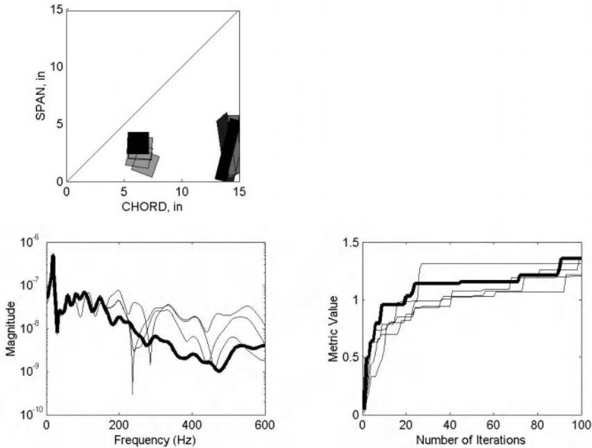
Figure 12.19. Optimization results for patches with maximum 2x2 inch actuators.
