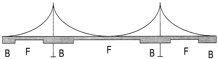
Figure 6.31. Schematic of Akashi-Kiokyo suspension bridge . Note spanwise non-uniformity of the deck shape. From M. Yamada, T. Miyata, N.N. Minh, H. Katsuchi, “Complex flutter-mode analysis for coupled gust response of the Akashi-Kaikyo Bridge model”, Wind Engineering into the 21st Century , Tenth Intern. Conf. on Wind Eng., A. Larsen, G.L. Larose, and F.M. Livesey (eds.), Vol. 2, Rotterdam:Bakkema, 1081-1088.
