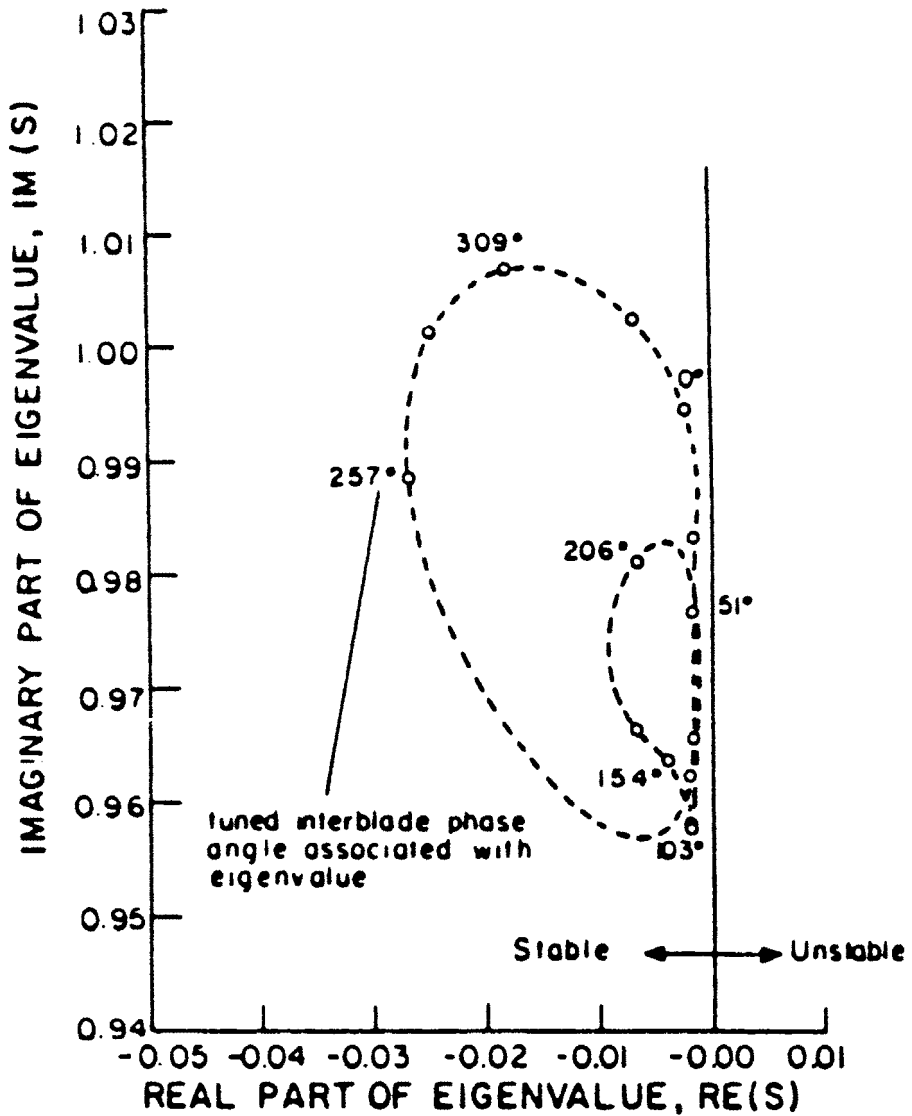
Figure 8.12b. Eigenvalues of the same rotor with 'optimal' mistuning.
