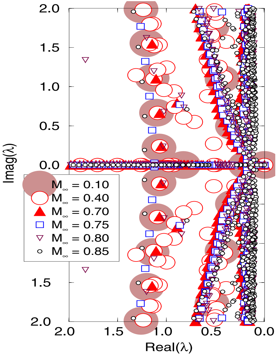
Figure 9.14. Real [ \text{Real}(\lambda) ] and imaginary [ \text{Imag}(\lambda) ] eigenvalues of unsteady flow about NACA 0012 airfoil for different Mach number ( M ) at zero angles of attack. (Republished from Florea et al (1999) with permission.)
