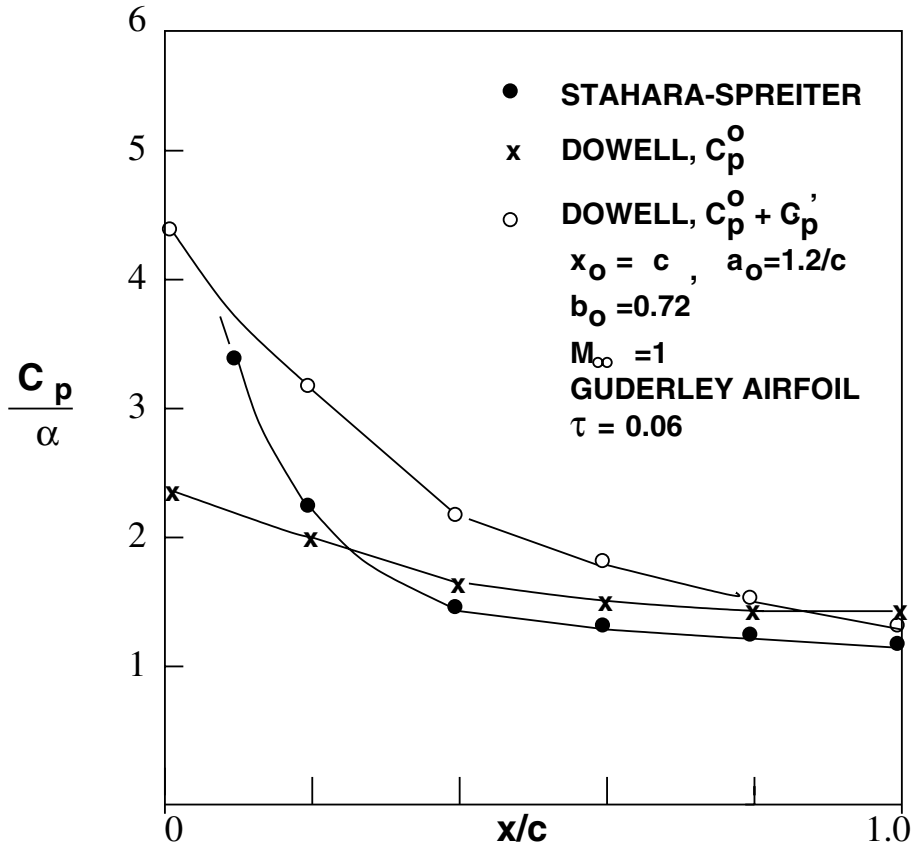
Figure 4.19. Pressure distribution for Guderley airfoil at constant angle of attack.
