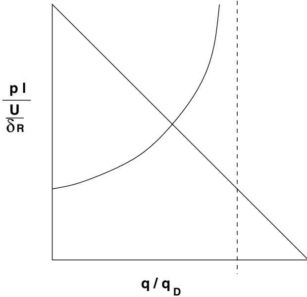
Figure 2.13. Roll rate vs dynamic pressure.
