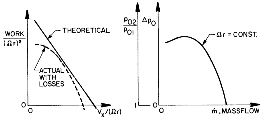
Figure 8.2. Work and pressure ratio relationships.
