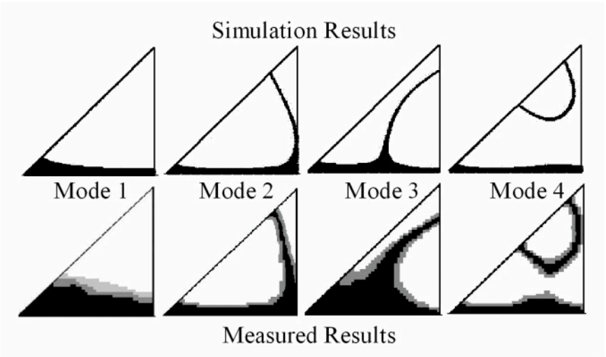
Figure 12.33. Comparison of predicted and measured delta wing mode shapes
