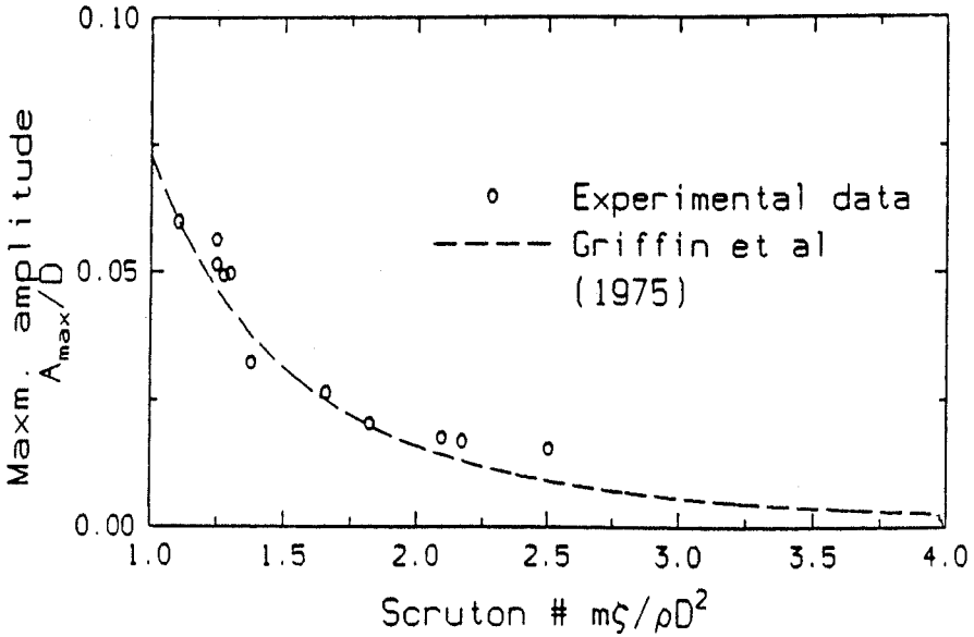
Figure 6.7. Maximum amplitude as a function of Scruton number.
