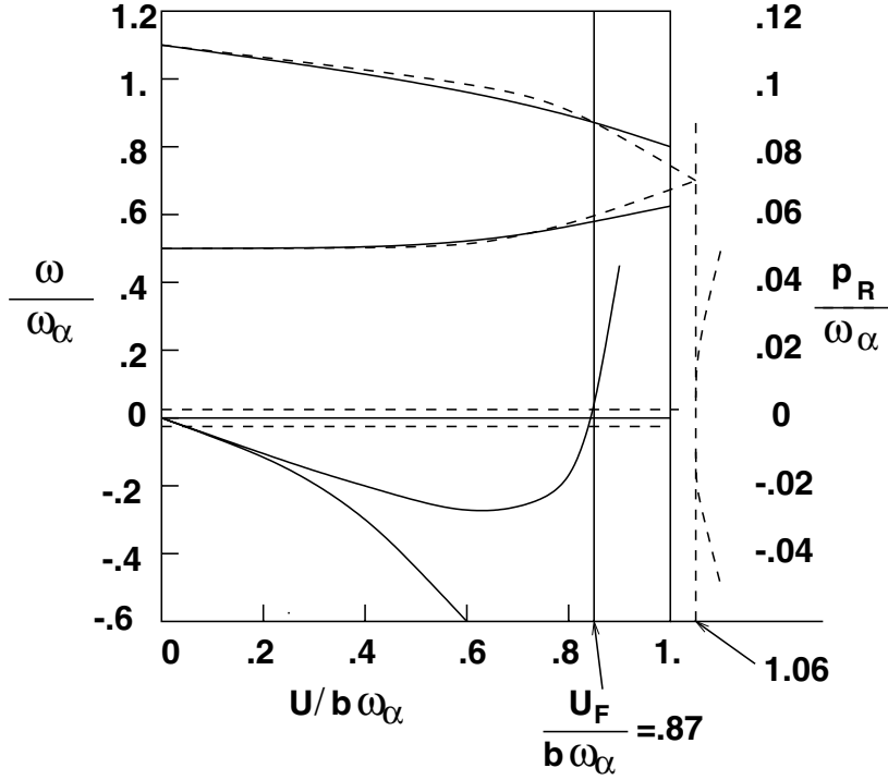
Figure 3.6. Dimensionless frequency \omega/\omega_\alpha and damping p_R/\omega_\alpha of the aeroelastic modes of the typical section, estimated using steady-state aerodynamic operators and plotted vs. reduced airspeed U/b\omega_\alpha . System parameters are x_\alpha = 0.05 , r_\alpha = 0.5 , \omega_h/\omega_\alpha = 0.5 , (2m/\pi\rho_\infty bS) = 10 , e/b = 0.4 , \frac{\partial C_L}{\partial \alpha} = 2\pi . Solid curves – with aerodynamic damping. Dashed curves – without aerodynamic damping.
